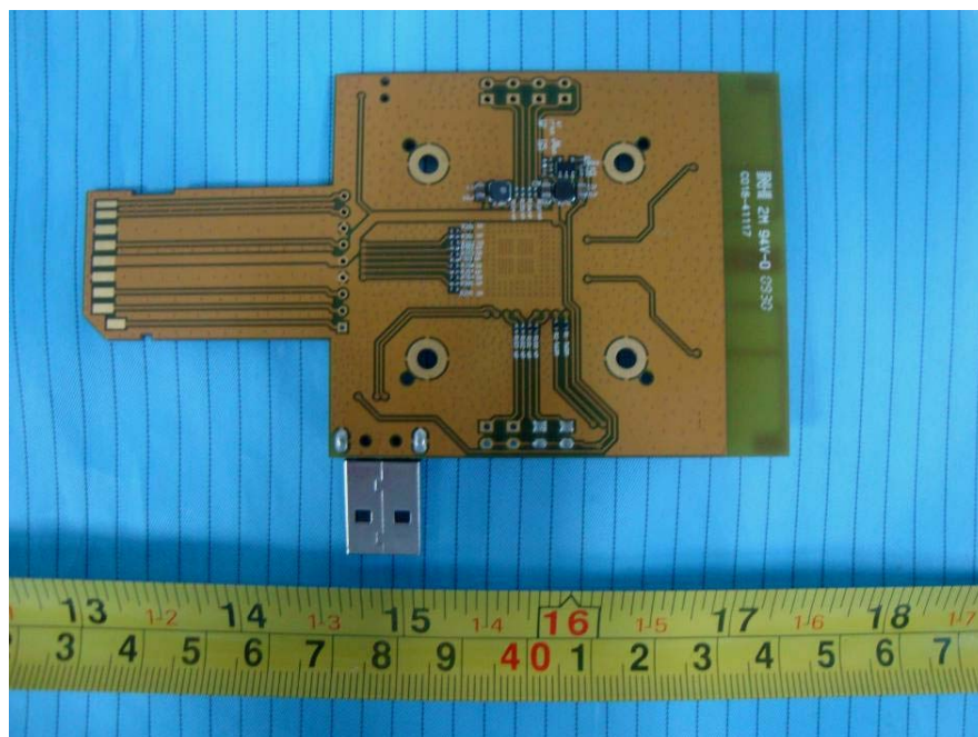
Supported Board Rear View
