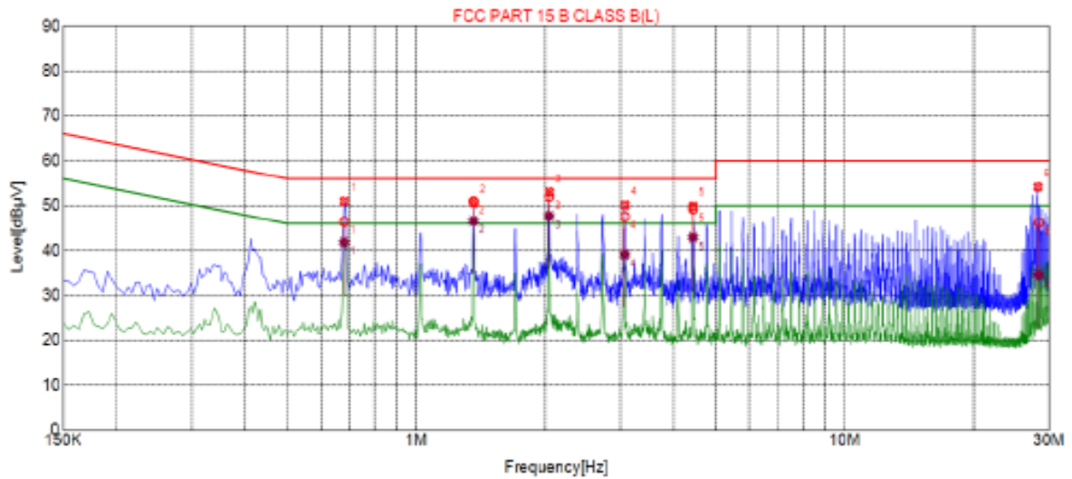
Line Conducted Emission Test Line 1-L
