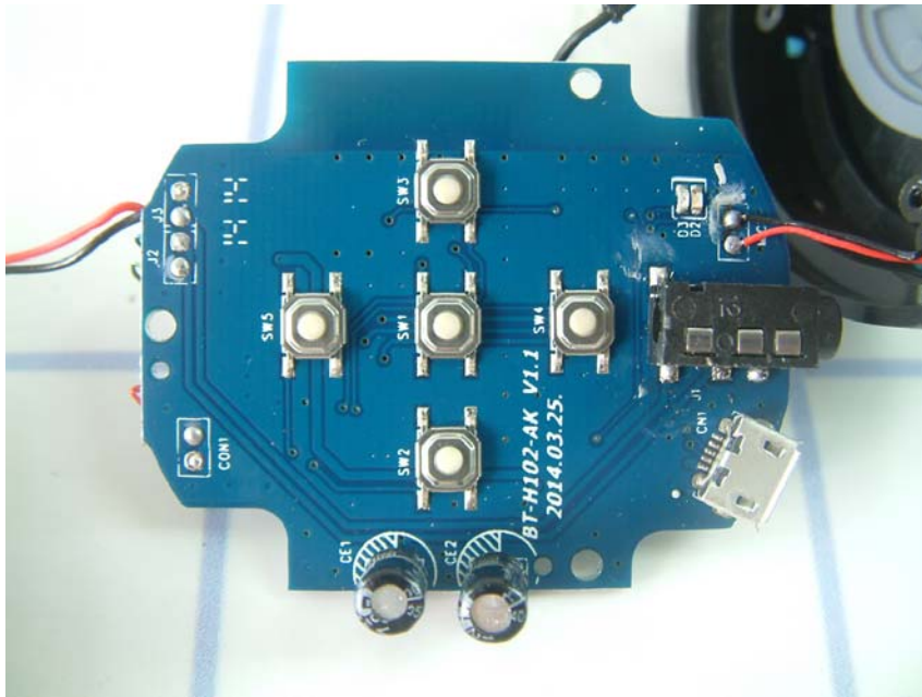
PCB view 1 side 2
