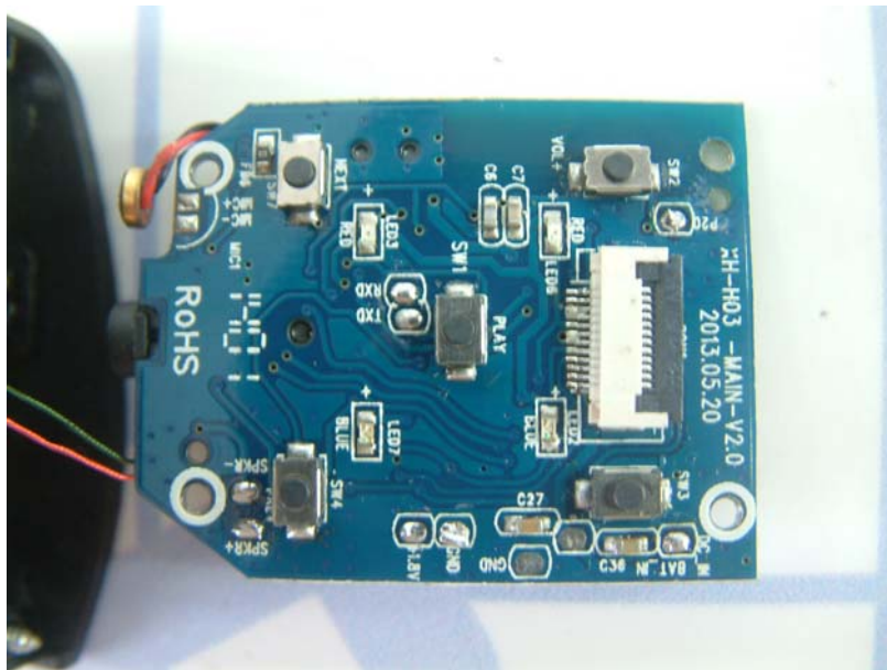
PCB view 2 side 2
