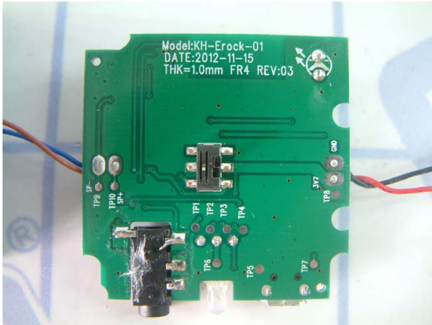
PCB view 1 side 1
