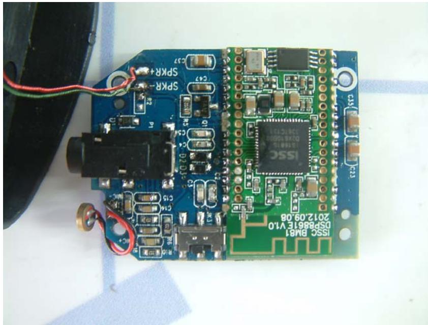
PCB view 2 side 1
