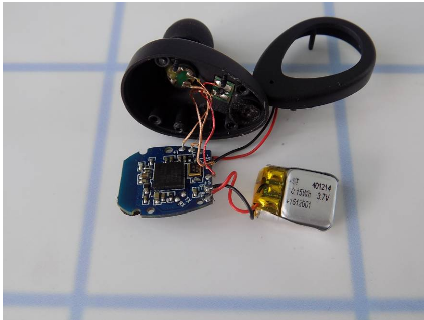
Internal view 3
