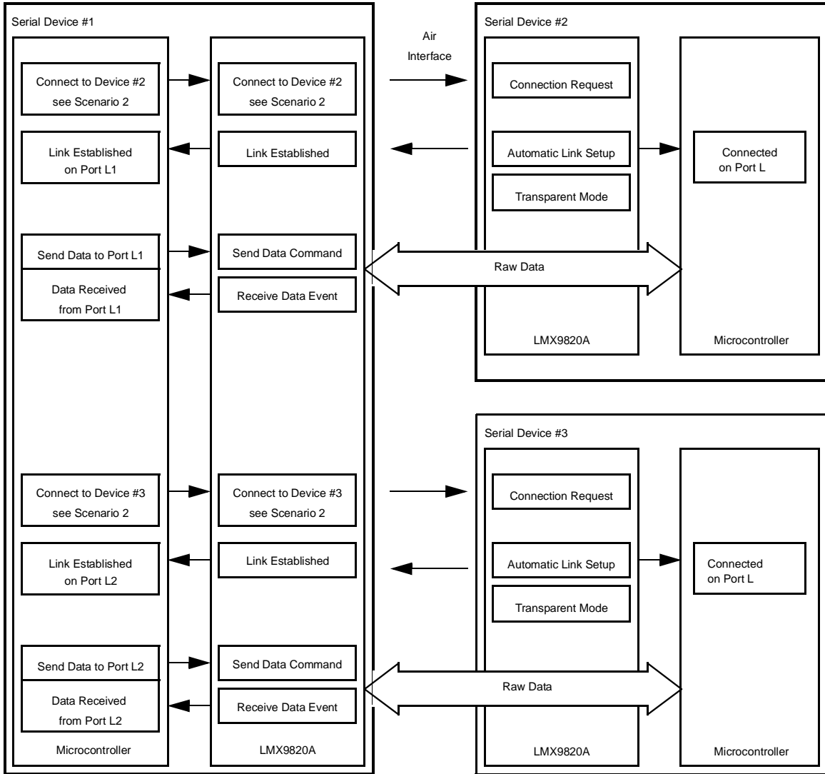
Figure 21. Point-to-Multipoint Connection
