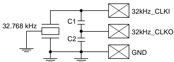
Figure 13. 32.768 kHz Oscillator
