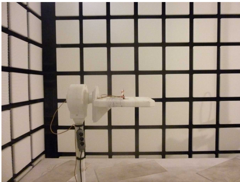
Photo 2: EUT at the anechoic chamber, stand-alone module with integrated antenna
