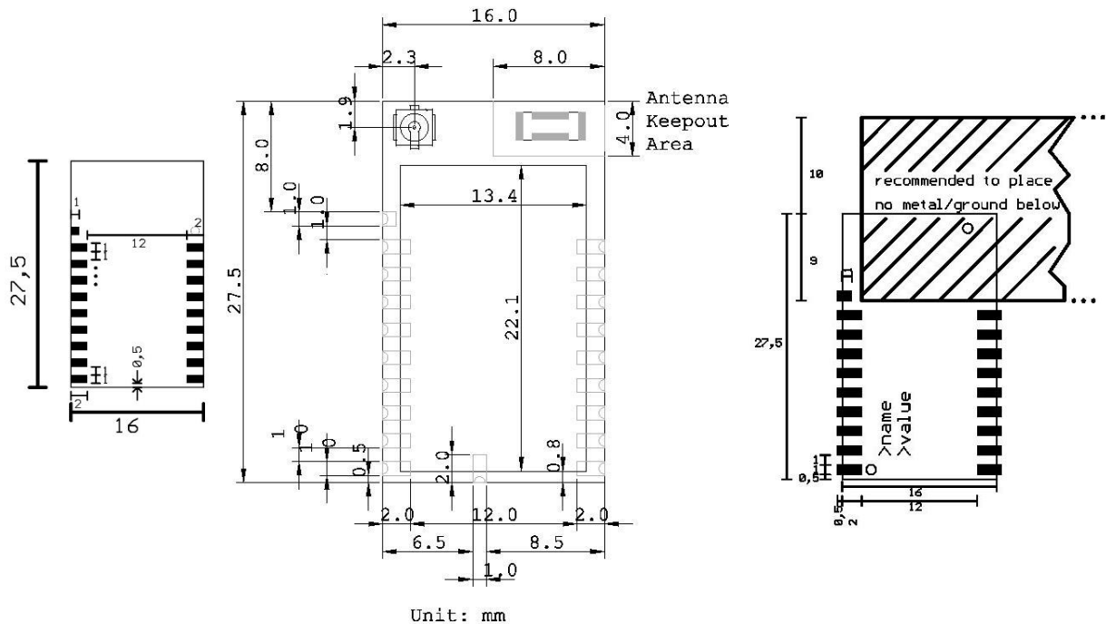
Figure 5 Dimensional drawing AMB8420
