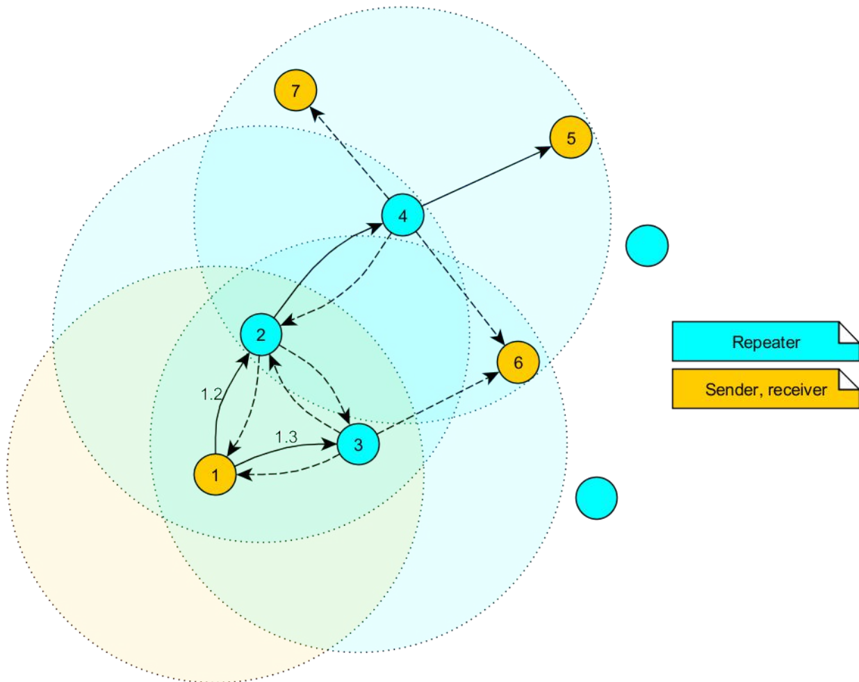
Figure 7: Example network
