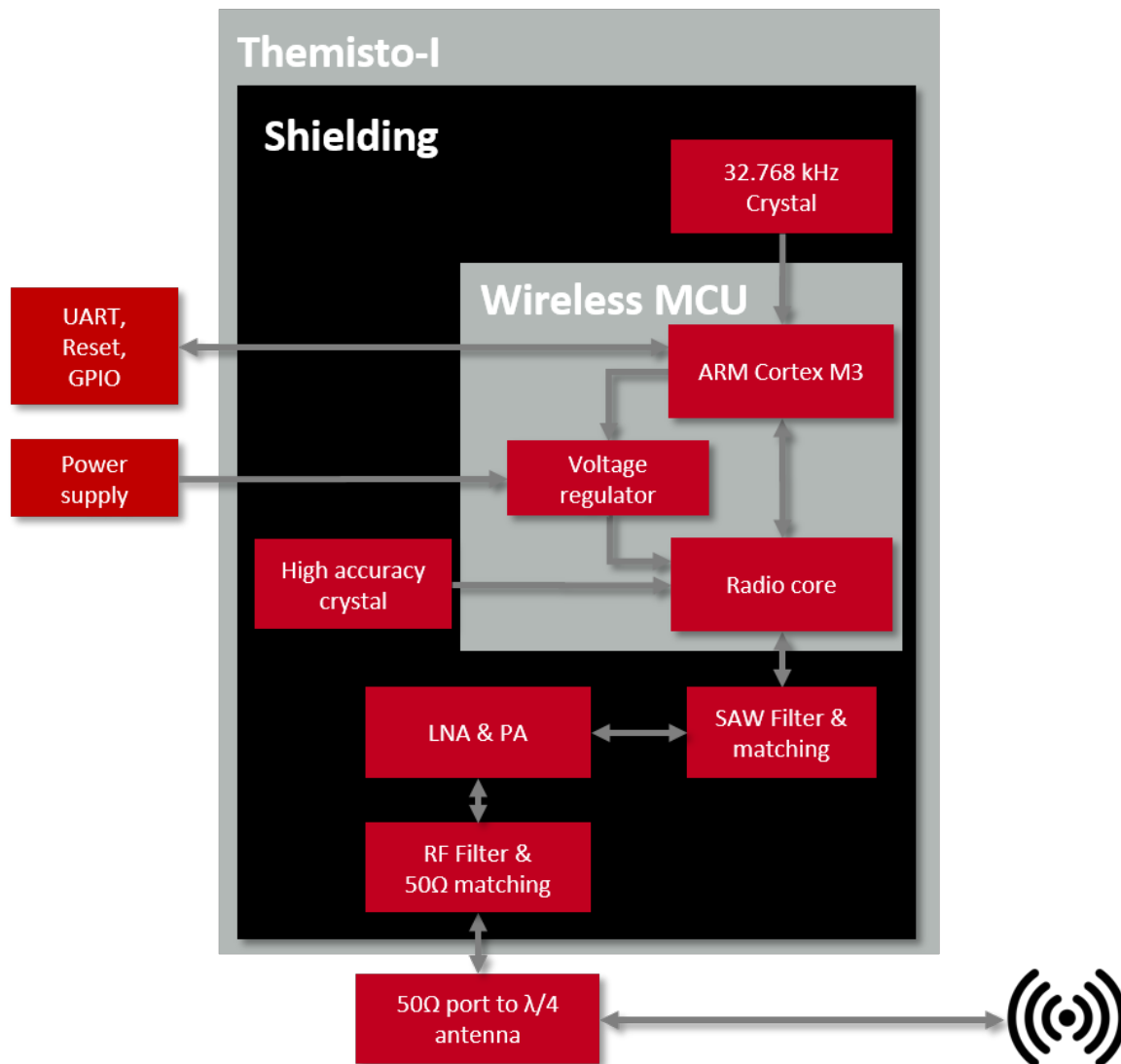
Figure 1: Block diagram
