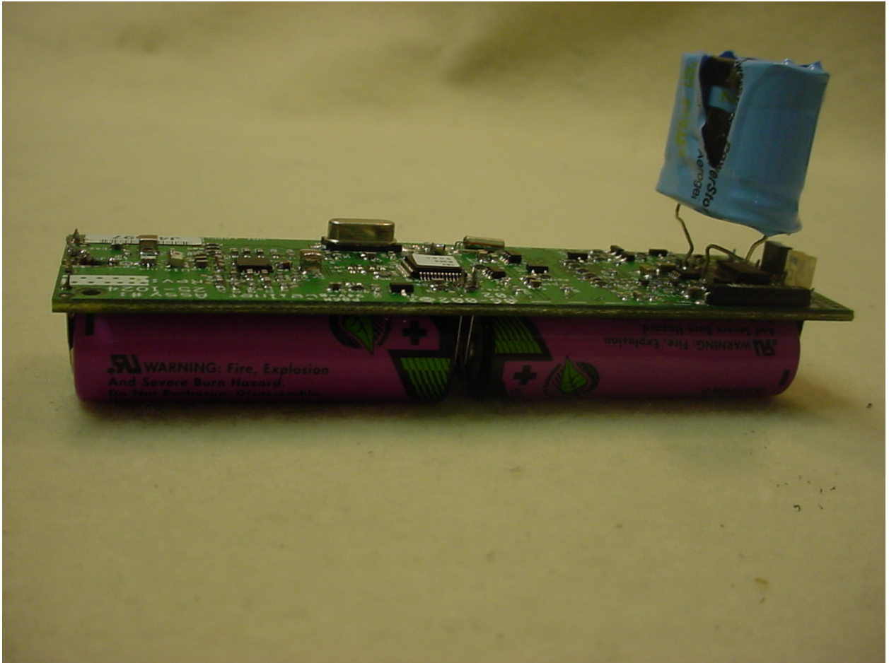
Figure 2: Internal – Side View
