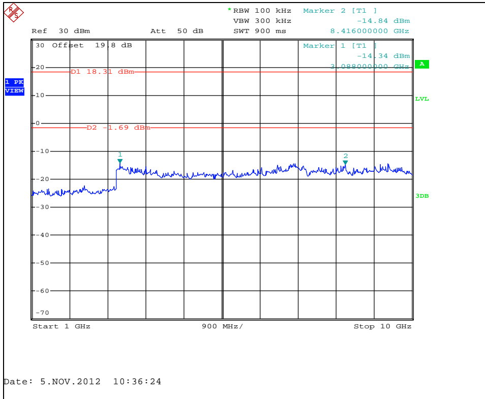
Figure 7.5.1.2-2: 1 GHz – 10 GHz
