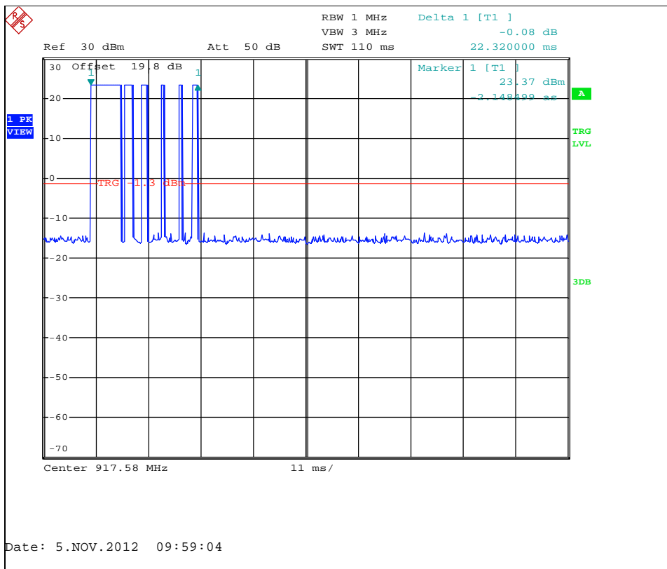
Figure 7.5.2.2-1: Duty Cycle
