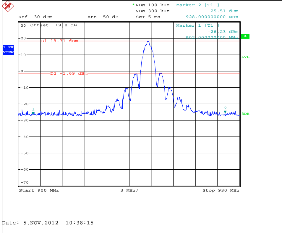
Figure 7.5.1.2-3: Band-edge (Conducted)
