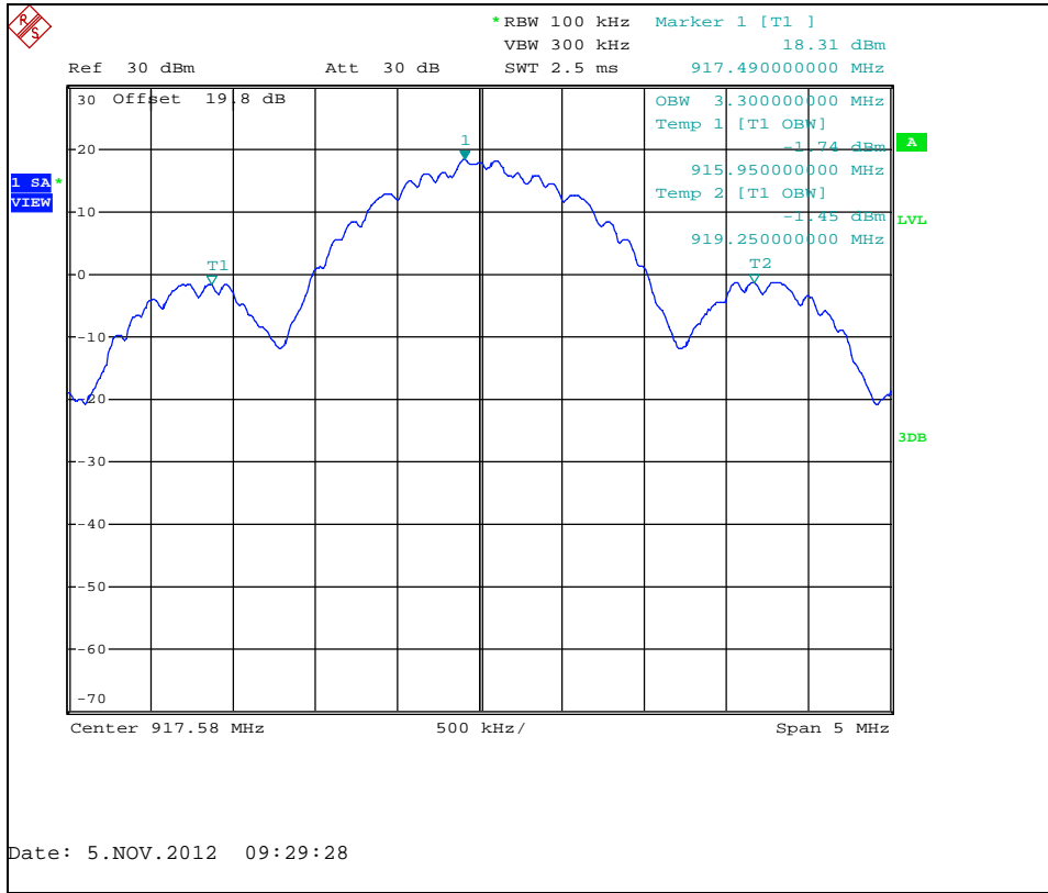
Figure 7.3.2-2: 99% Bandwidth Plot
