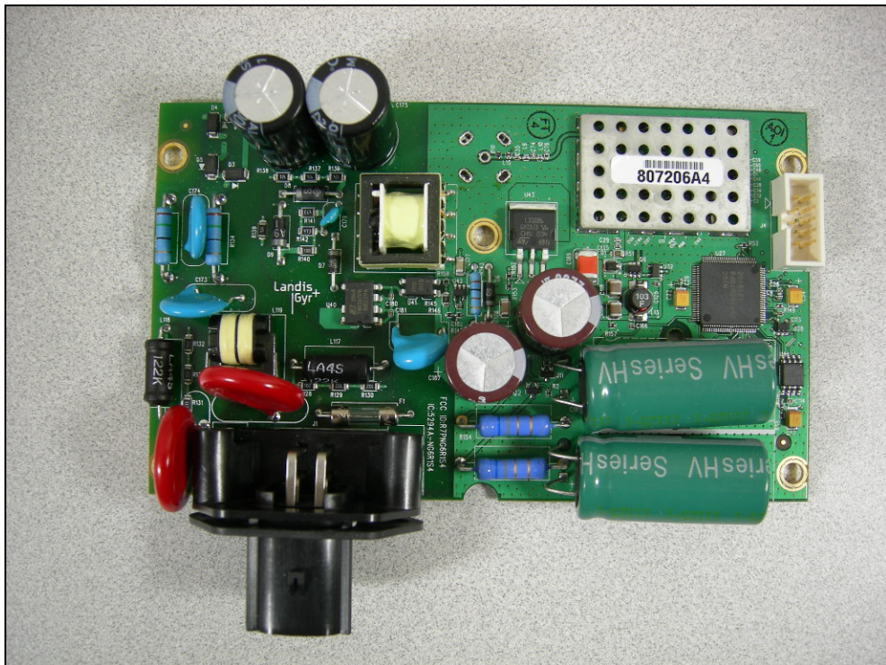
Figure 2: Internal Photo – With Shield
