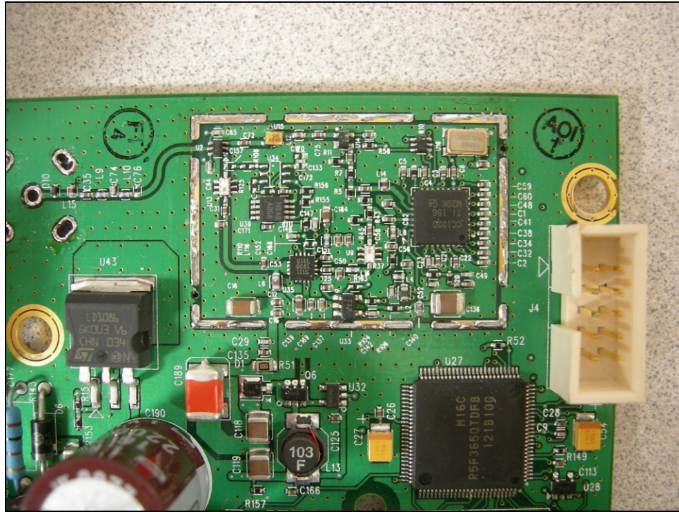
Figure 3: Internal Photo – Without Shield
