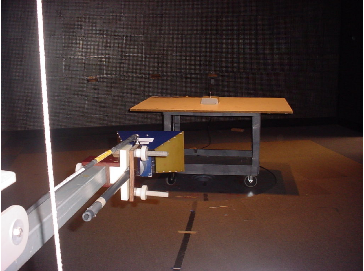
Figure 6: Radiated Emissions - Intentional
