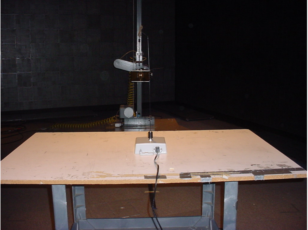
Figure 5: Radiated Emissions - Intentional
