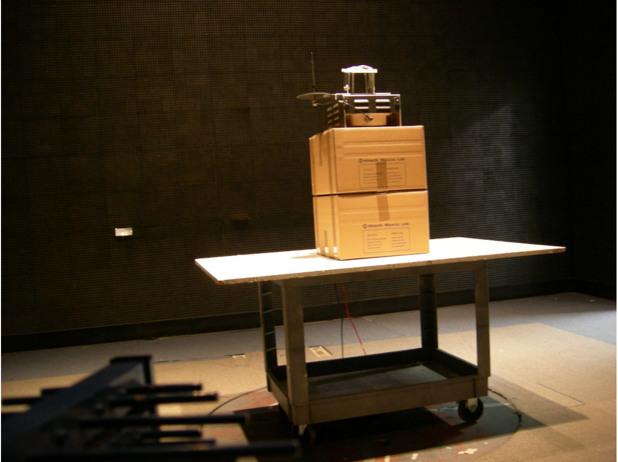
Figure 3: Radiated Emissions (Arm Mount Hardware)
