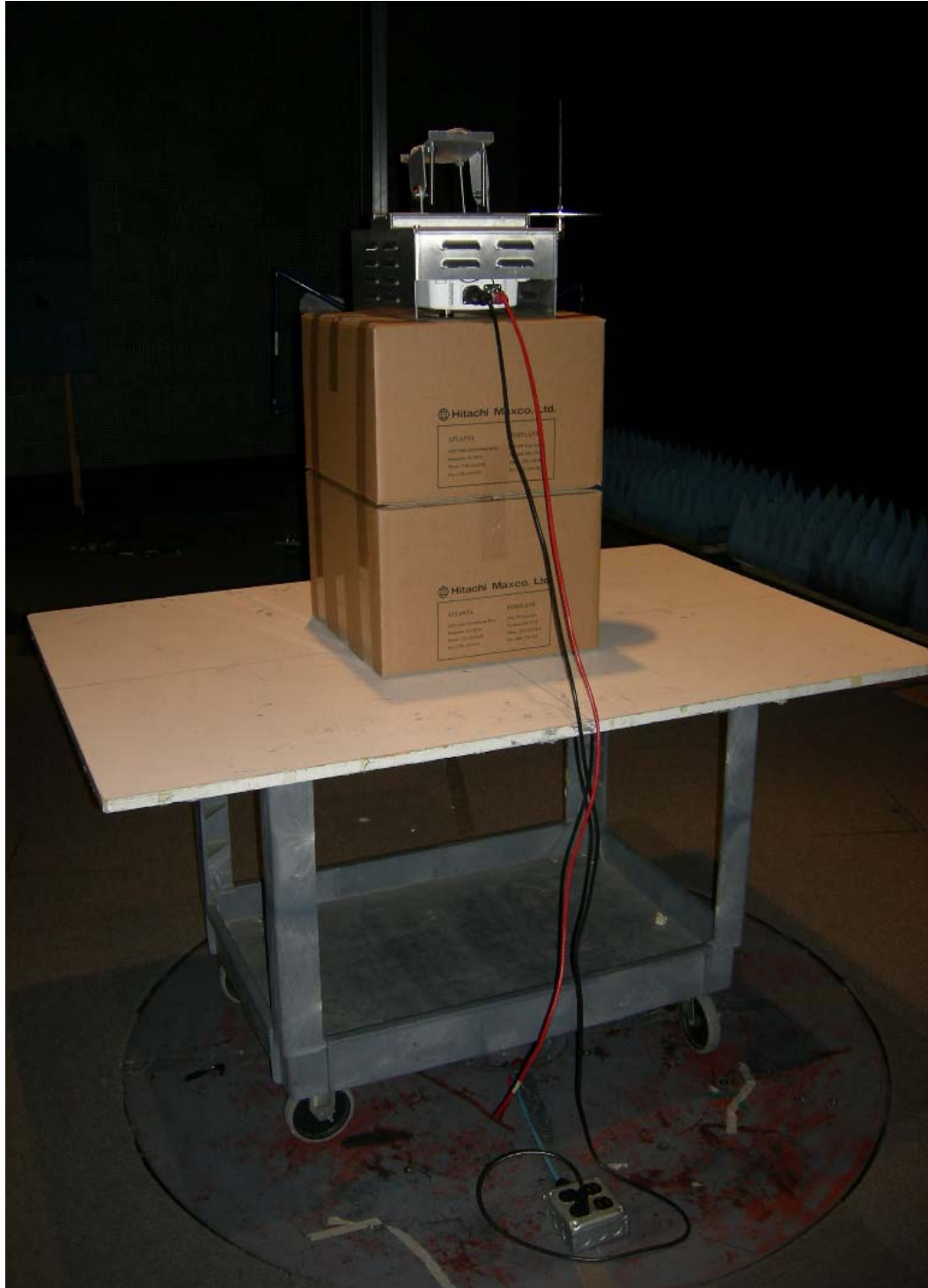
Figure 4: Radiated Emissions (Arm Mount Hardware)
