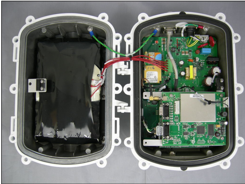
Figure 5: PCB – Installed
