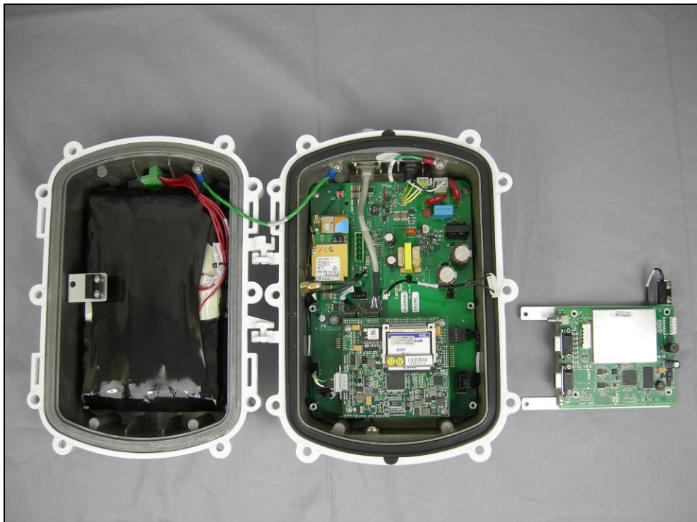
Figure 4: PCB - Installation
