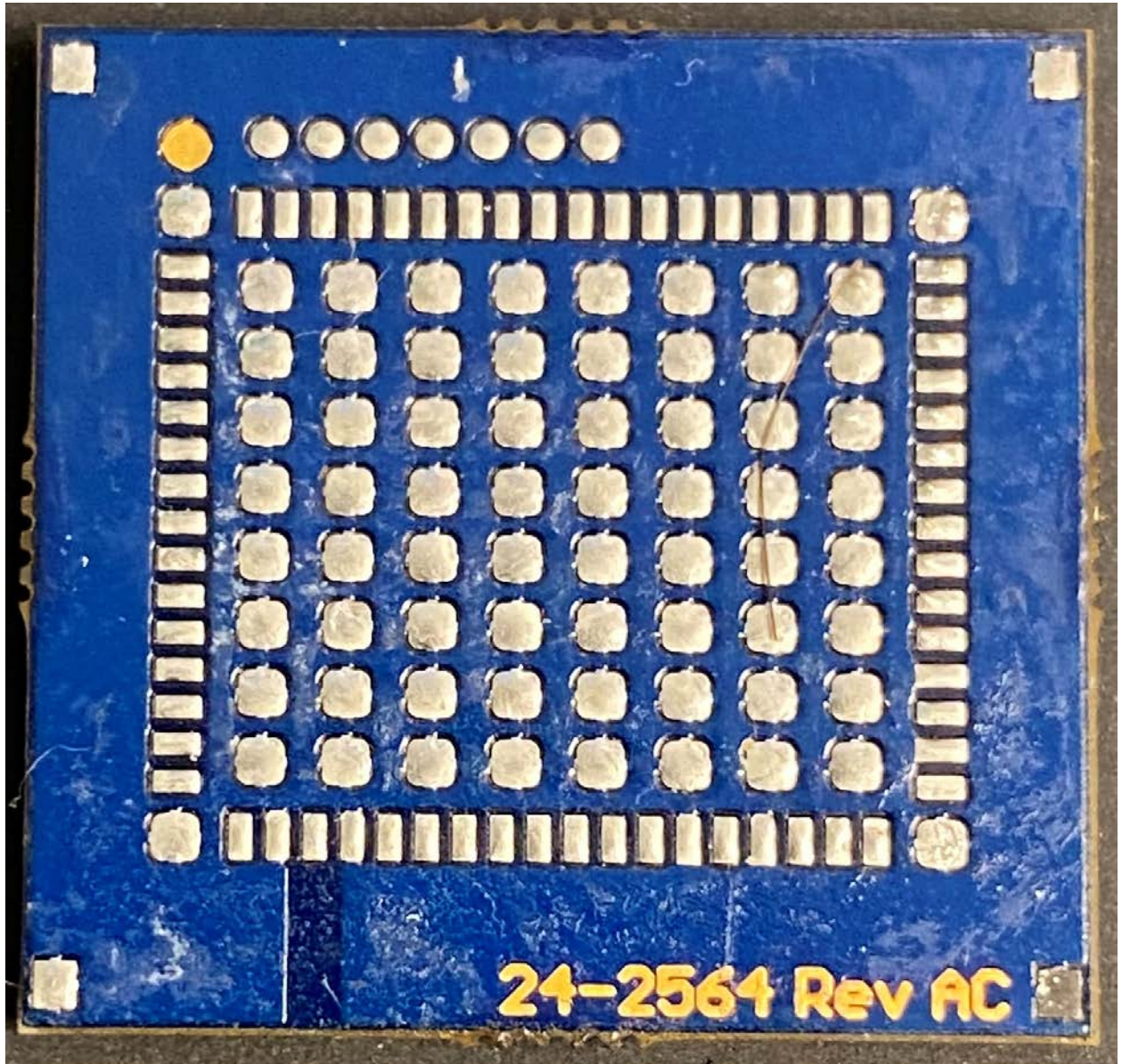
Figure 2: Bottom View
