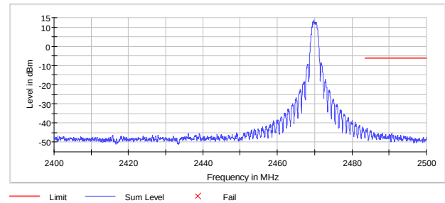
Figure 7.5.1.2-5: Upper Band-edge (Ch 24 @ TX PWR -1)
