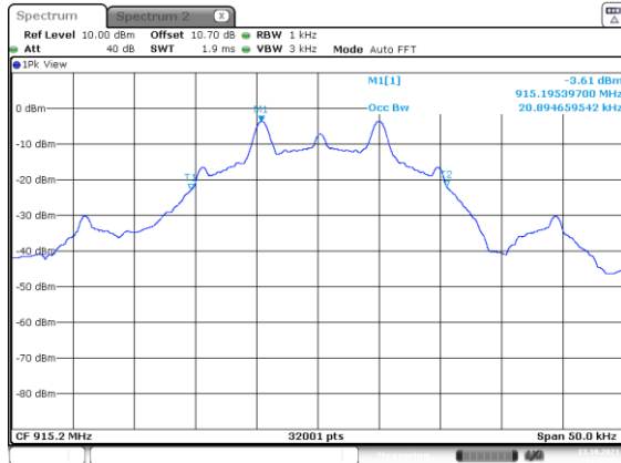
Figure 2.3.6-17: 99% BW Mid Channel – 9.6 kbps
