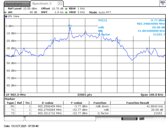
Figure 2.3.6-2: 20dB BW Low Channel – 19.2 kbps
