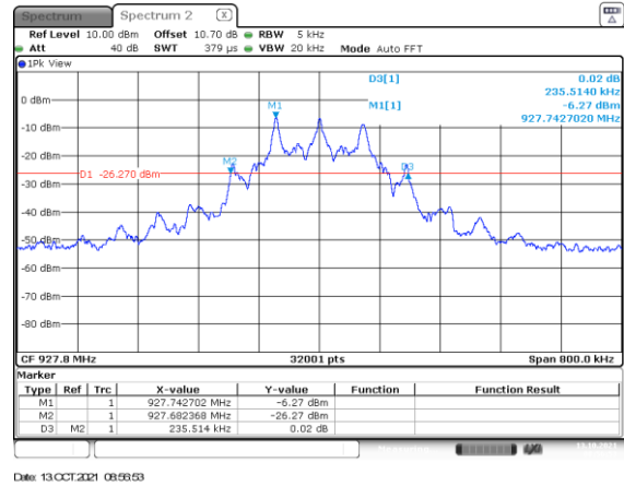
Figure 2.3.6-12: 20dB BW High Channel – 115.2 kbps
