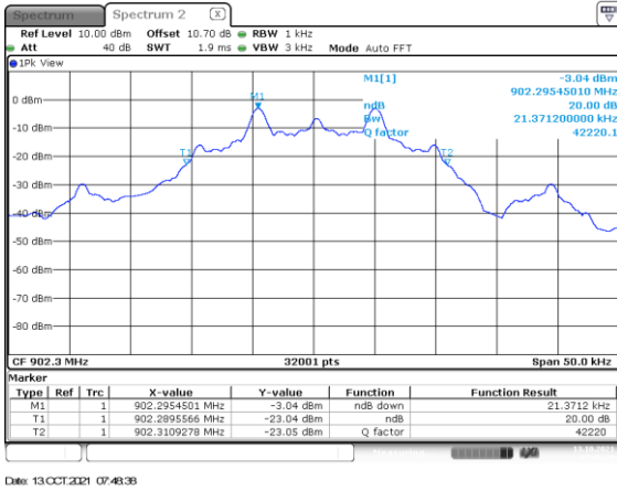
Figure 2.3.6-1: 20dB BW Low Channel – 9.6 kbps
