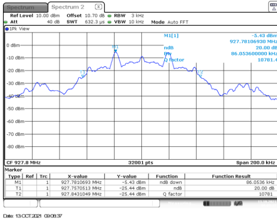
Figure 2.3.6-11: 20dB BW High Channel – 38.4 kbps
