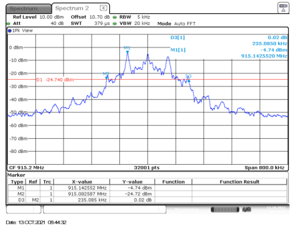
Figure 2.3.6-8: 20dB BW Mid Channel – 115.2 kbps
