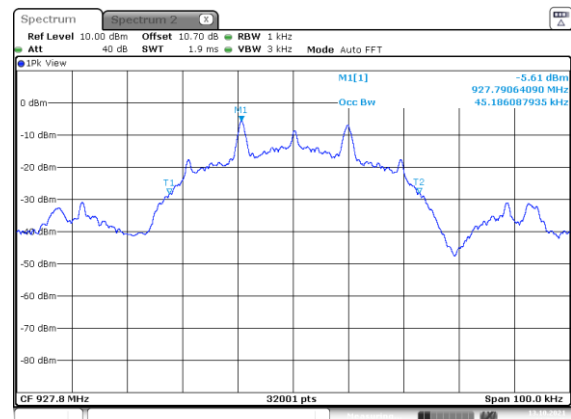
Figure 2.3.6-20: 99% BW Mid Channel – 115.2 kbps
