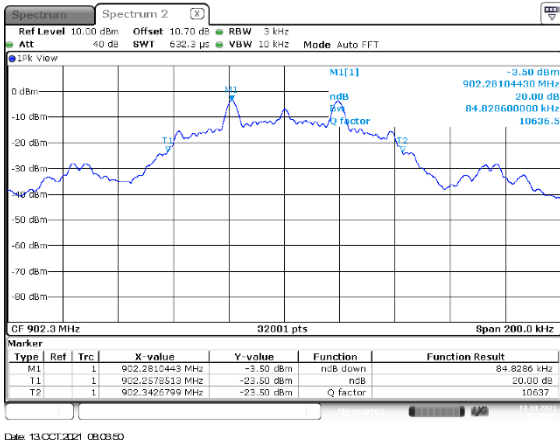
Figure 2.3.6-3: 20dB BW Low Channel – 38.4 kbps
