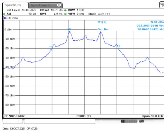
Figure 2.3.6-13: 99% BW Low Channel – 9.6 kbps
