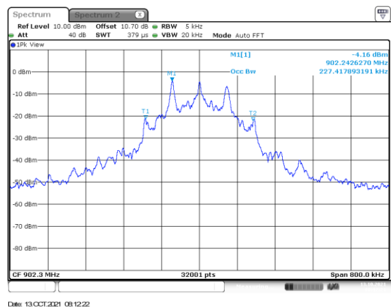
Figure 2.3.6-16: 99% BW Low Channel – 115.2 kbps
