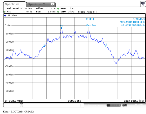
Figure 2.3.6-14: 99% BW Low Channel – 19.2 kbps
