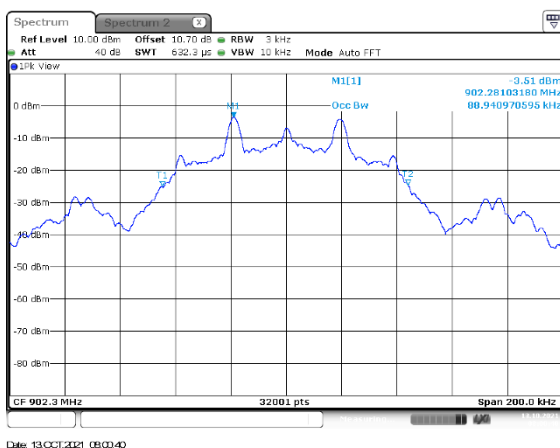
Figure 2.3.6-15: 99% BW Low Channel – 38.4 kbps
