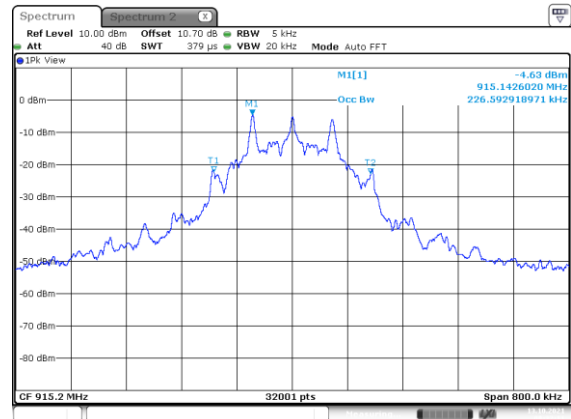
Figure 2.3.6-18: 99% BW Mid Channel – 19.2 kbps
