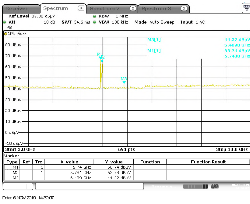
Figure A-6: Radiated Emissions – 3GHz-10GHz
