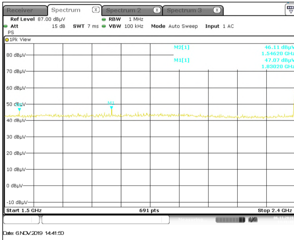
Figure A-4: Radiated Emissions – 1.5GHz-2.4GHz
