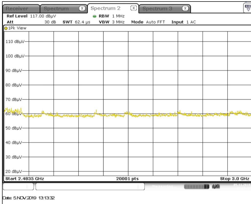
Figure A-4: Radiated Emissions – 2.4835GHz-3GHz
