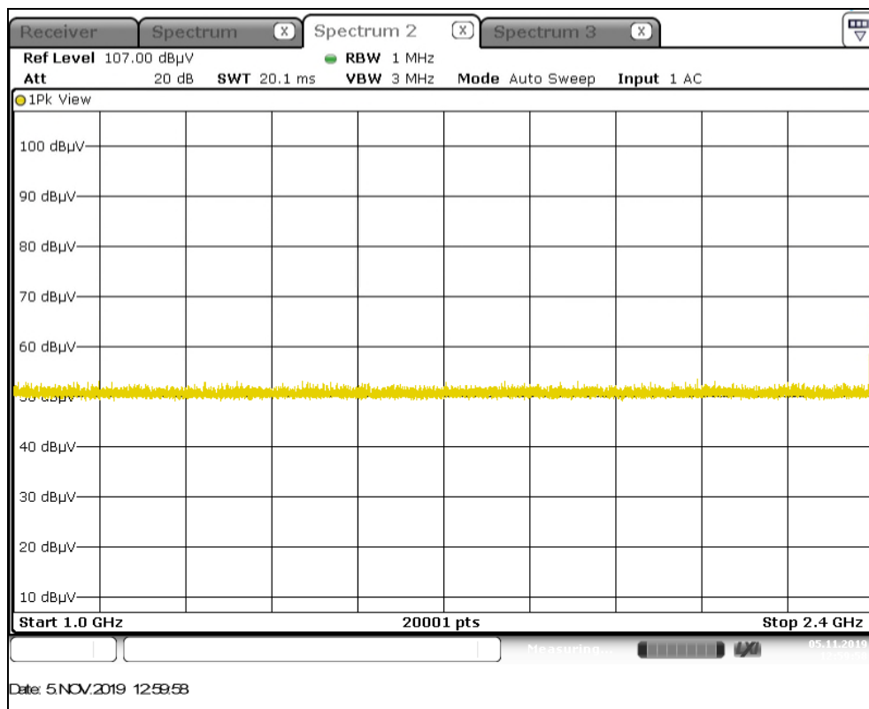
Figure A-4: Radiated Emissions – 1GHz-2.4GHz
