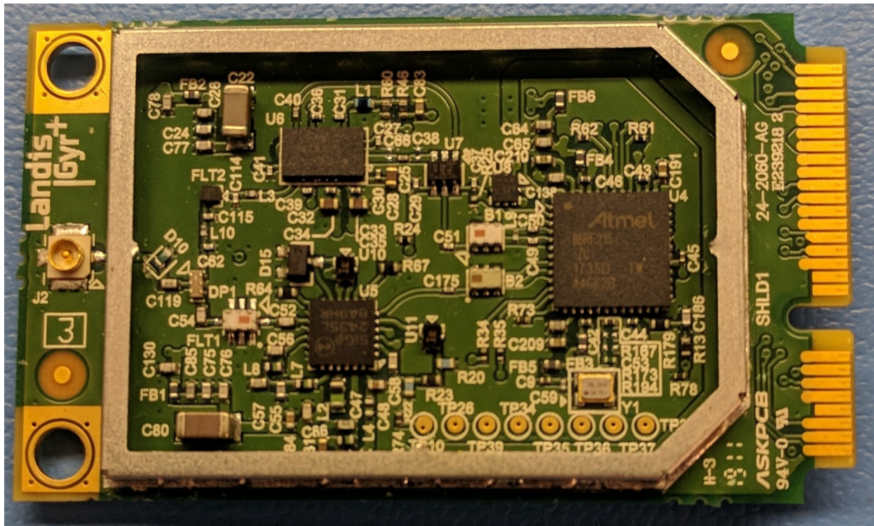
Figure 1: Top View
