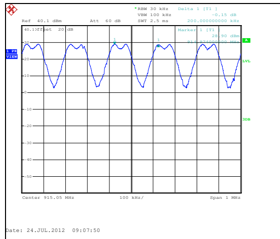
Figure 7.4.1.2-3: SUN Mode
