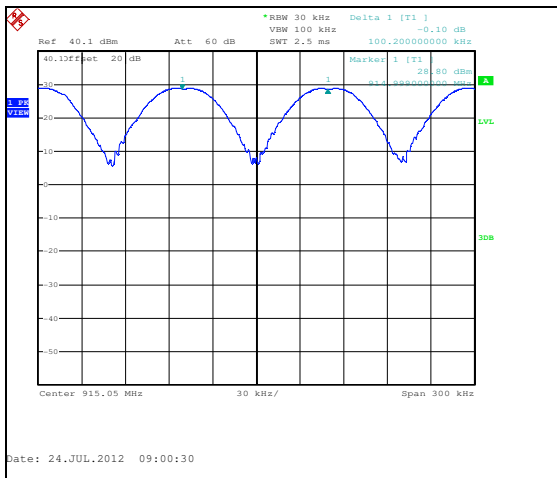
Figure 7.4.1.2-1: Narrow Mode
