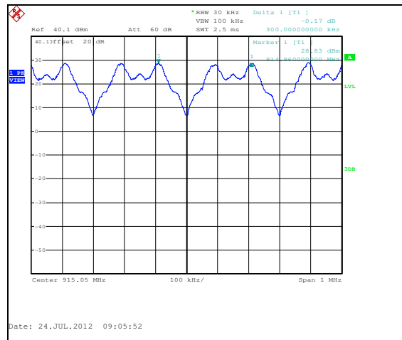
Figure 7.4.1.2-2: Wide Mode
