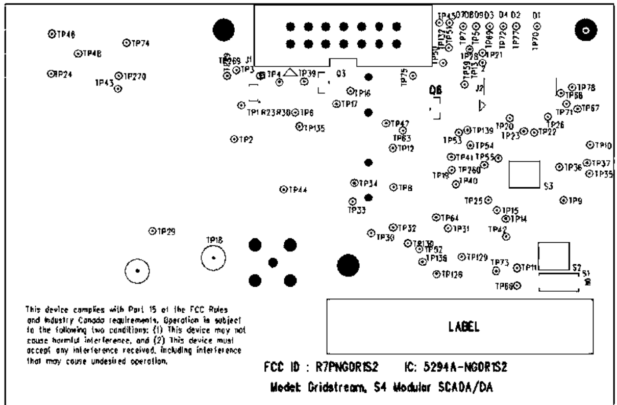
Figure 2: Label Placement – Internal Antenna
