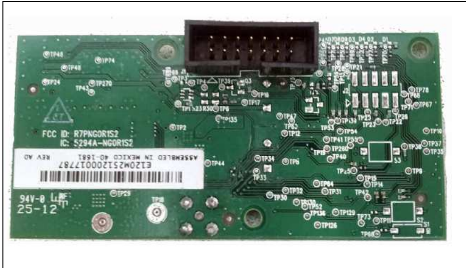
Figure 5: Internal Photo – External Antenna PCB – Back
