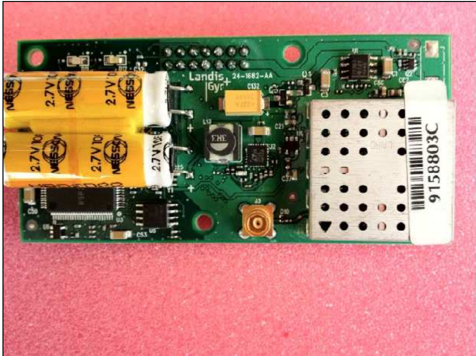
Figure 1: Internal Photo – External Antenna PCB with Shields
