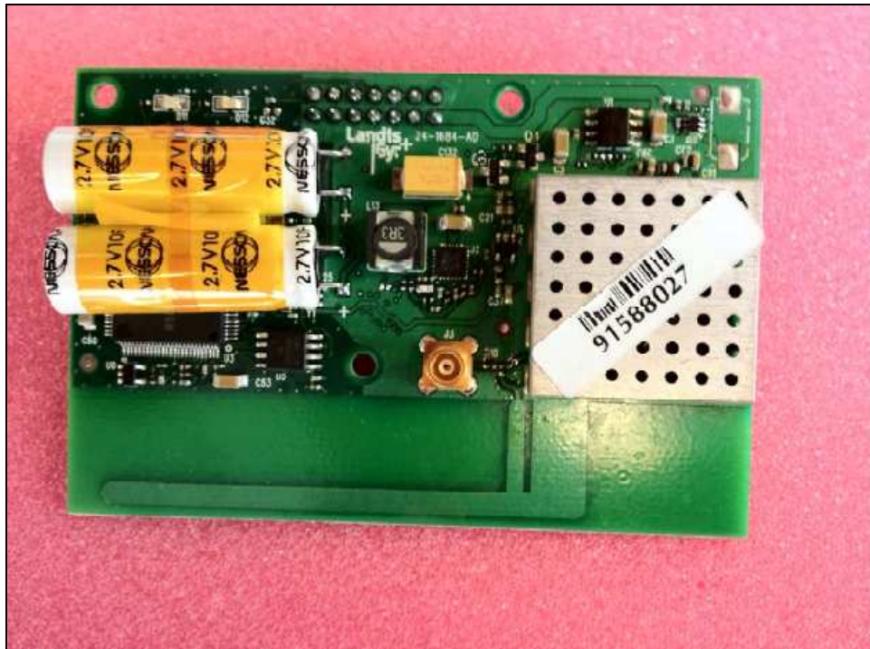
Figure 2: Internal Photo – Internal Antenna PCB with Shields
