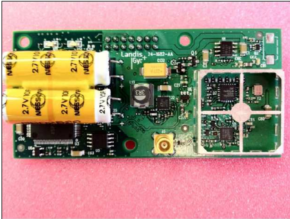
Figure 3: Internal Photo – External Antenna PCB without Shields
