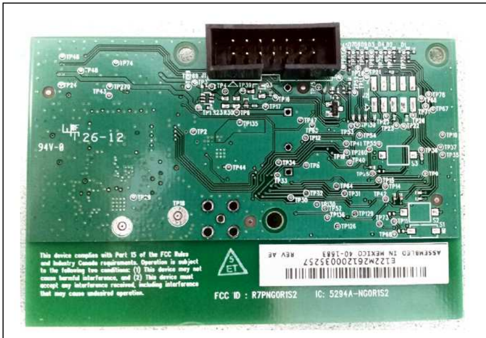
Figure 6: Internal Photo – Internal Antenna PCB – Back
