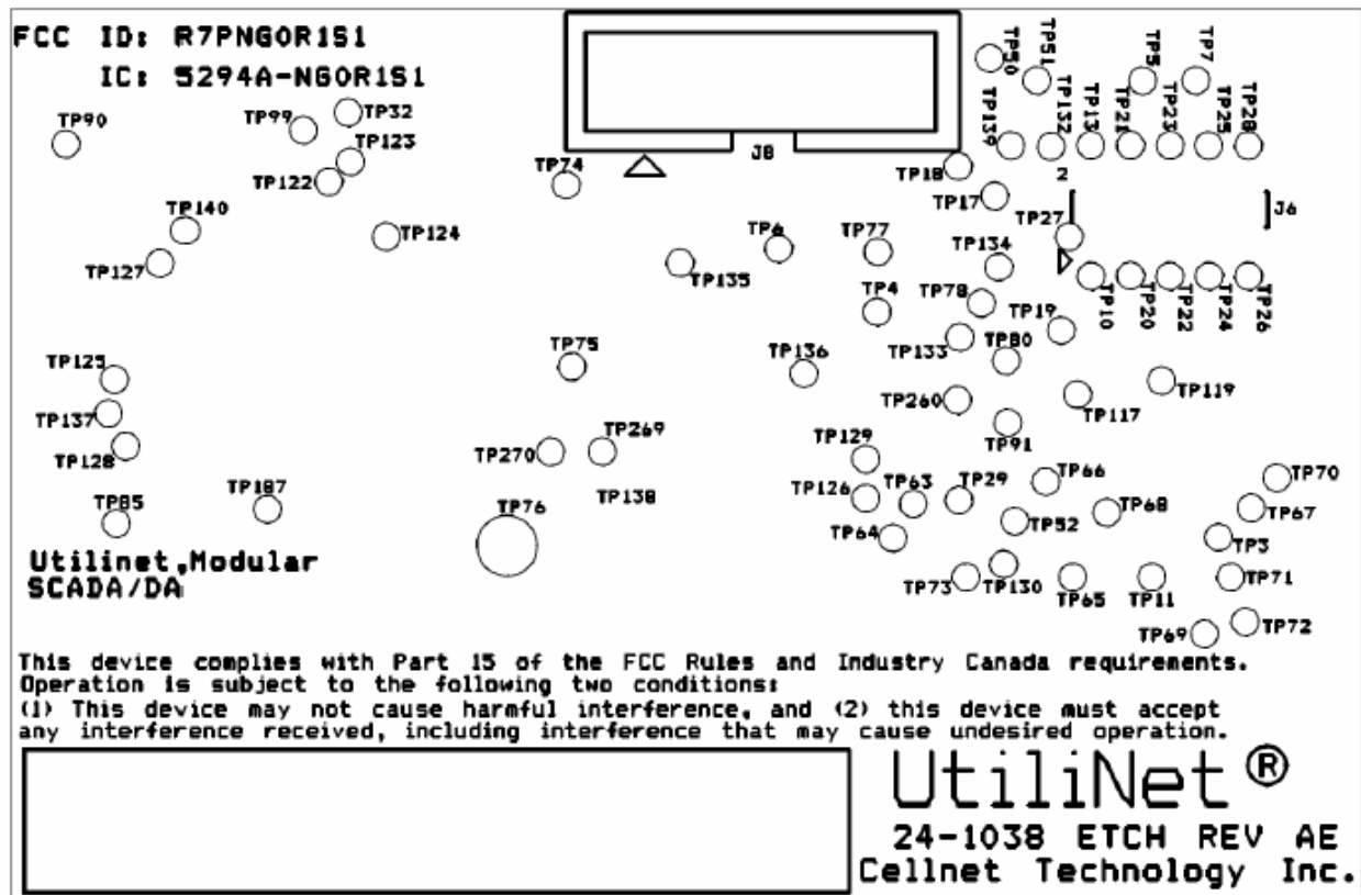
Figure 2: Internal Antenna Module – Label Sample and Location
