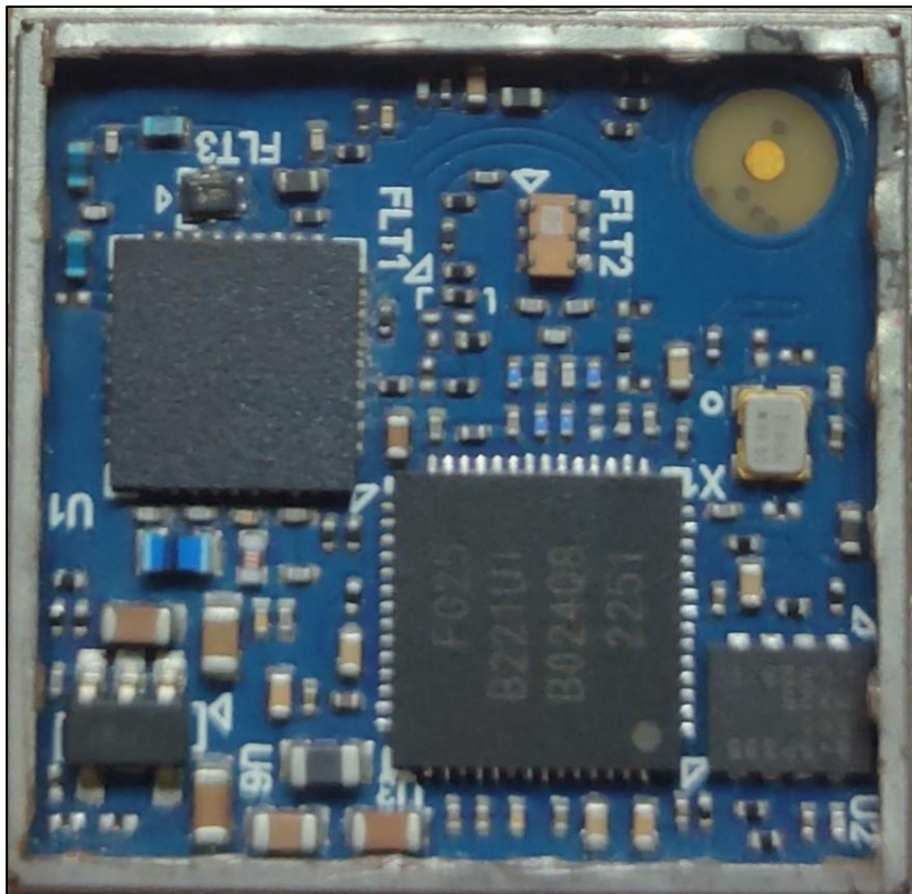
Module Without Shield
