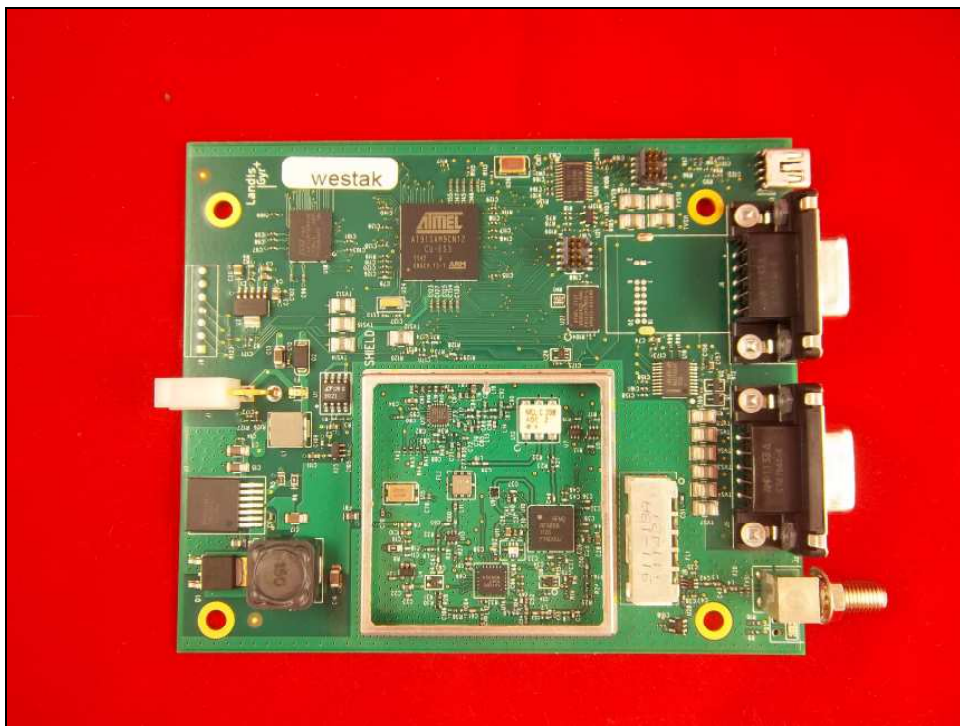
Figure 1: PCB without Shields
