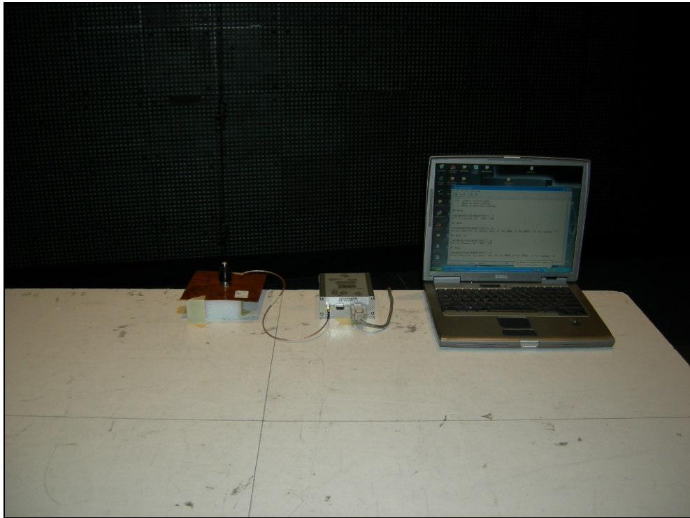
Figure 1: Radiated Emissions – Test Setup Photo
