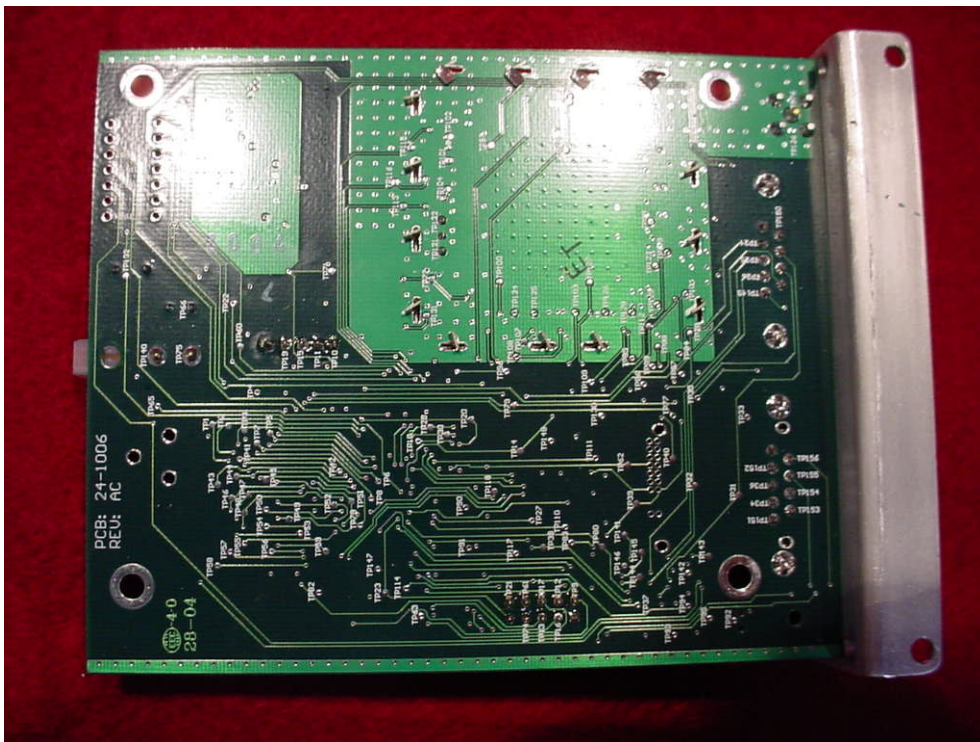
Figure 2: PCB Rear
