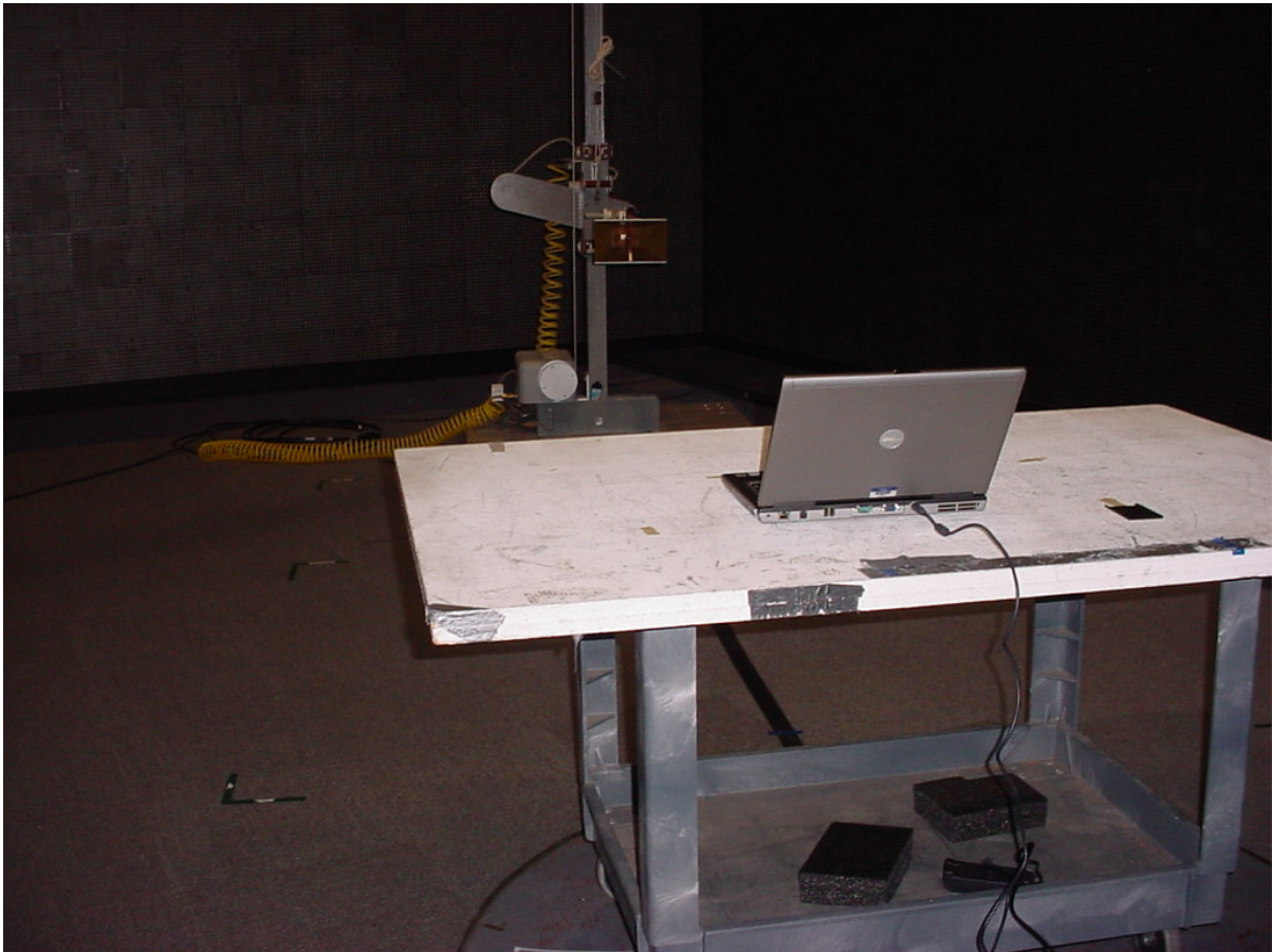
Figure 1: Test Setup - Radiated Emissions – Laptop Configuration
