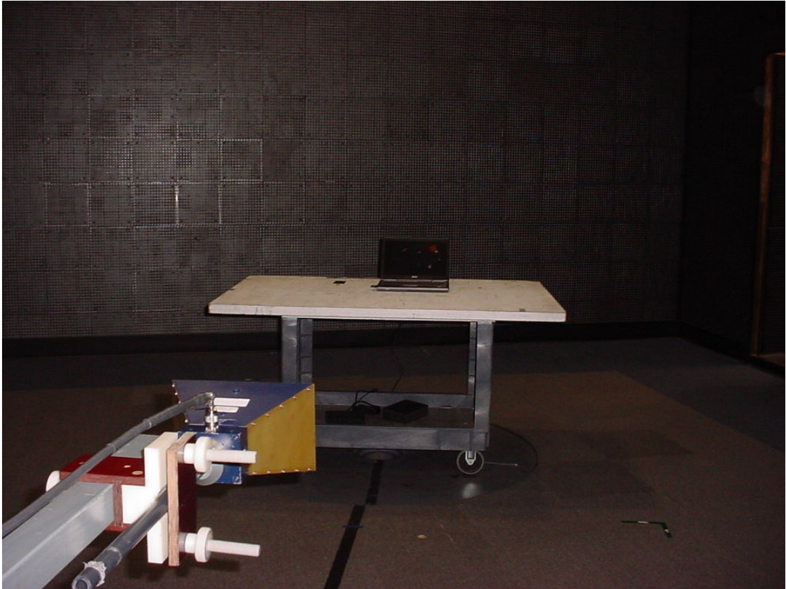
Figure 2: Test Setup - Radiated Emissions - Laptop Configuration
