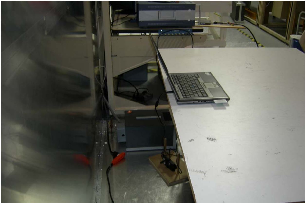
Figure 7: Test Setup - Conducted Emissions
