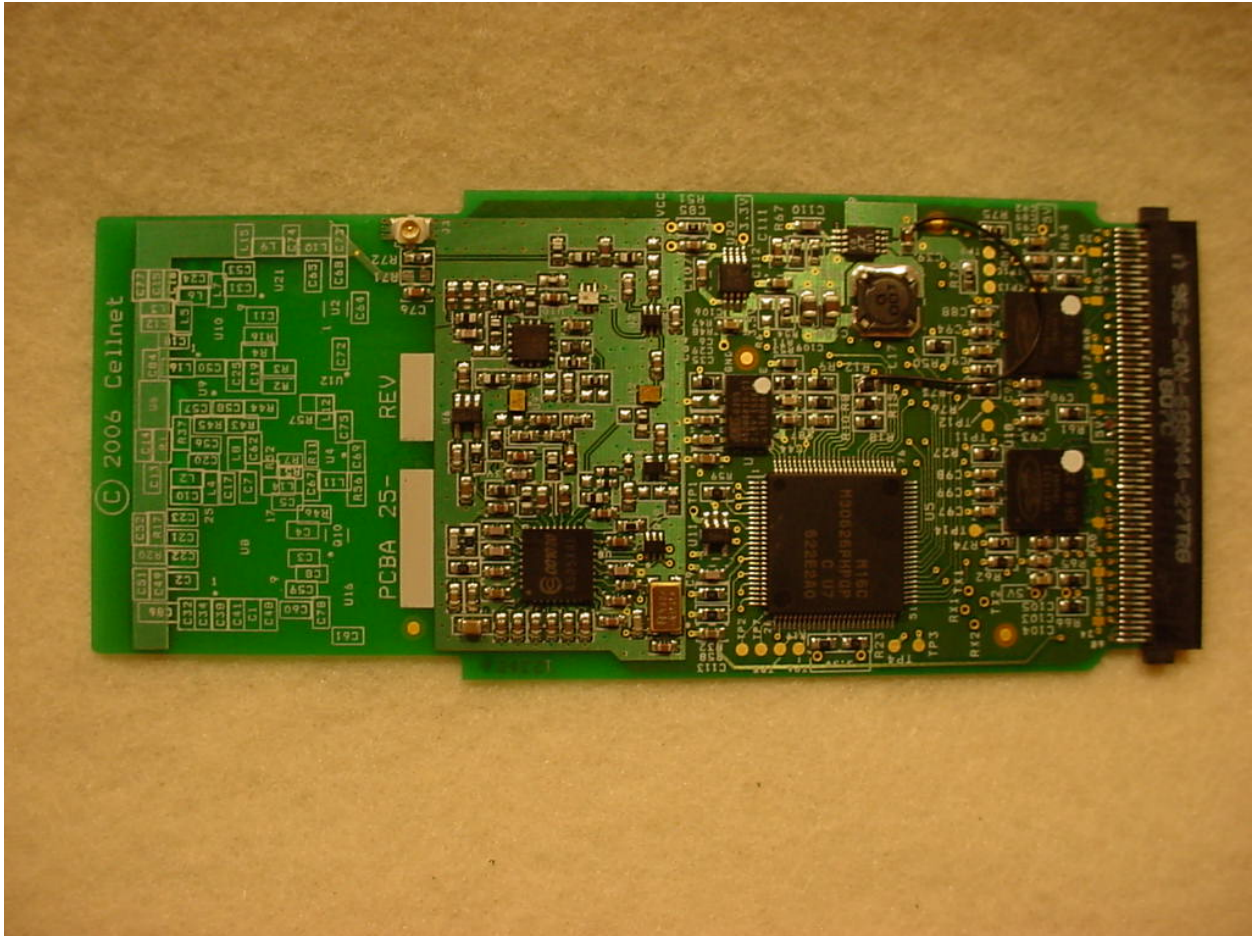
Figure 1: Internal Photos – PCB Front
