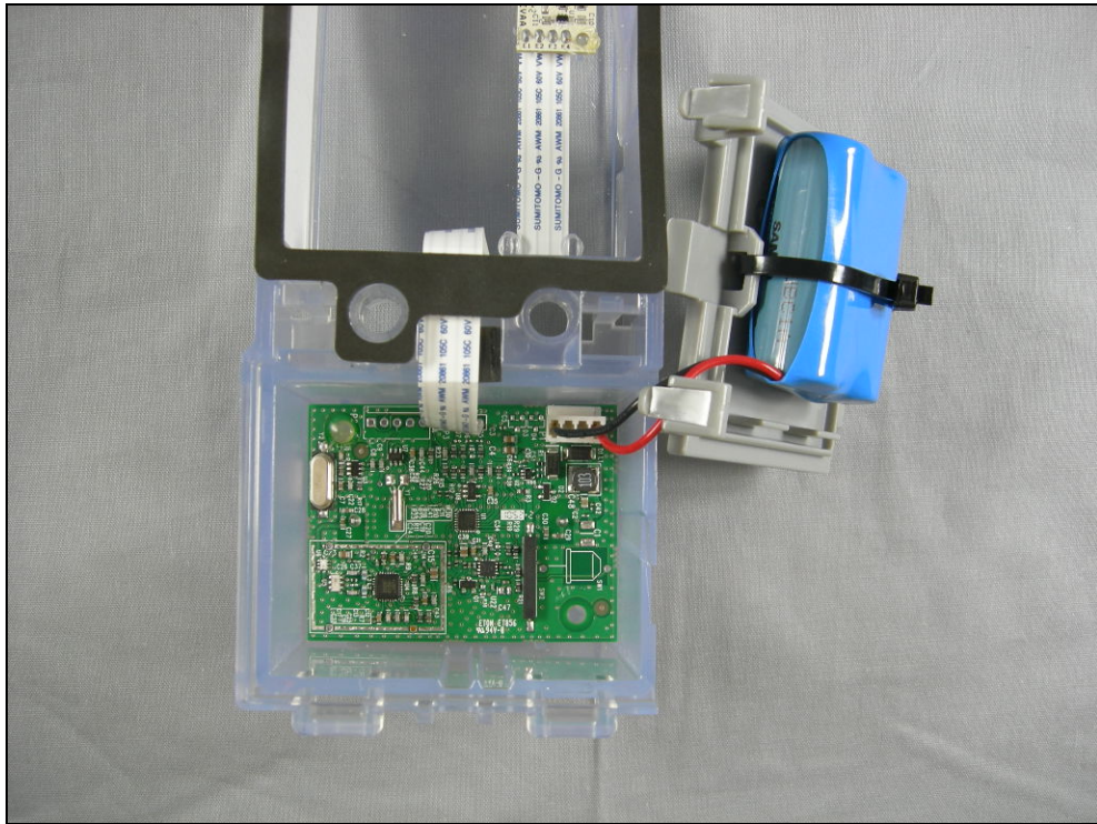
Figure 1: PCB Installed
