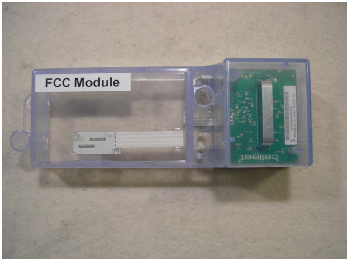
Figure 1: External – Front
