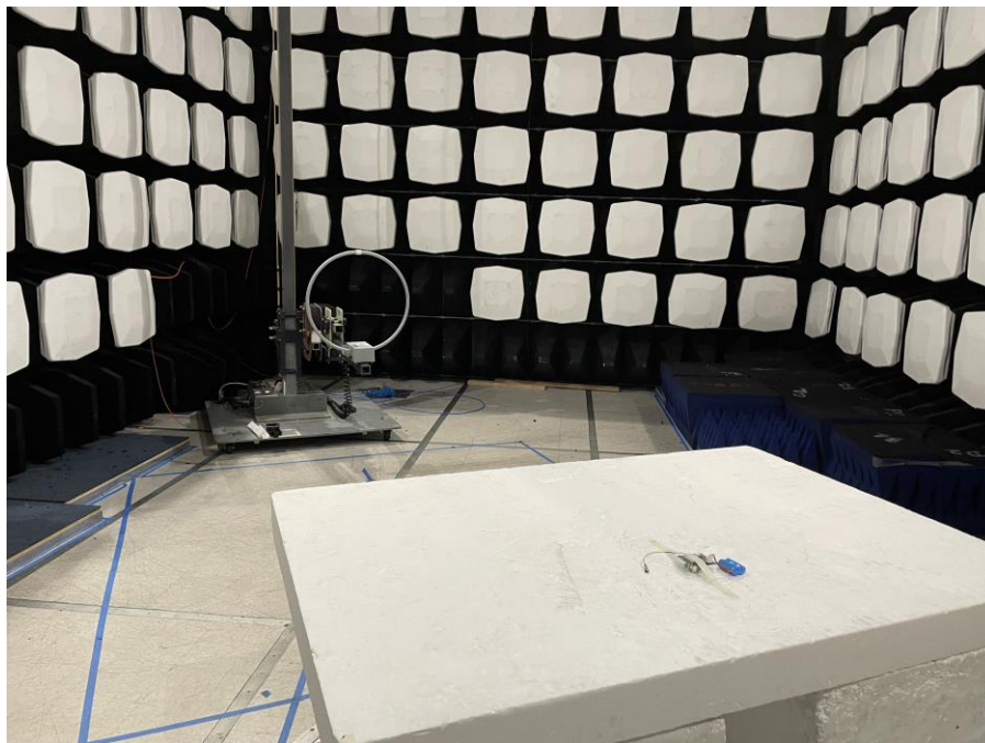
Figure 2: Equipment Under Test – Radiated Emissions <30MHz
