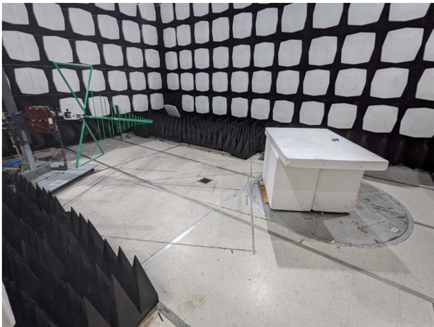
Figure 4: Equipment Under Test – Radiated Emissions <1GHz
