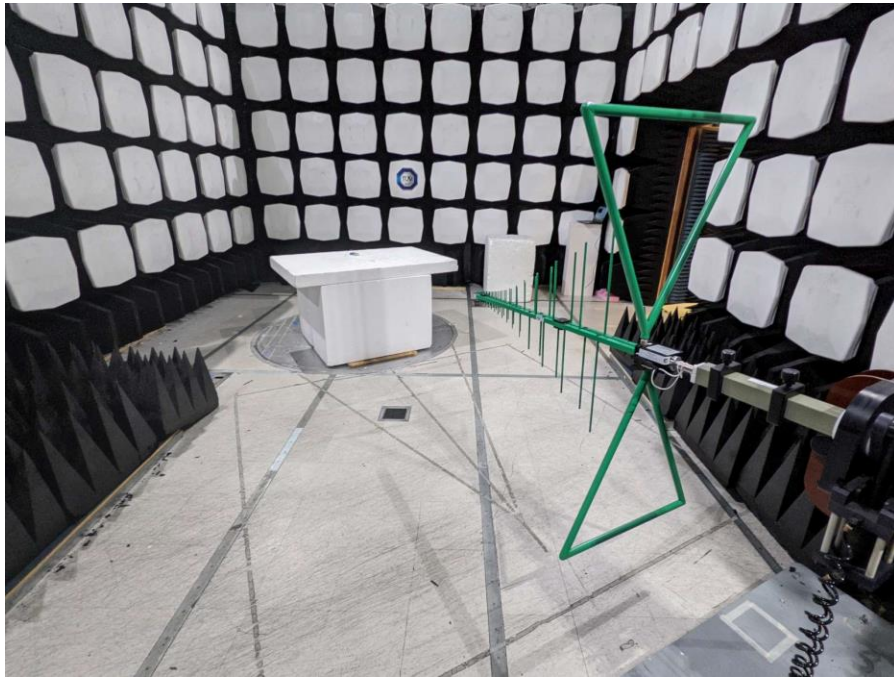
Figure 3: Equipment Under Test – Radiated Emissions <1GHz
