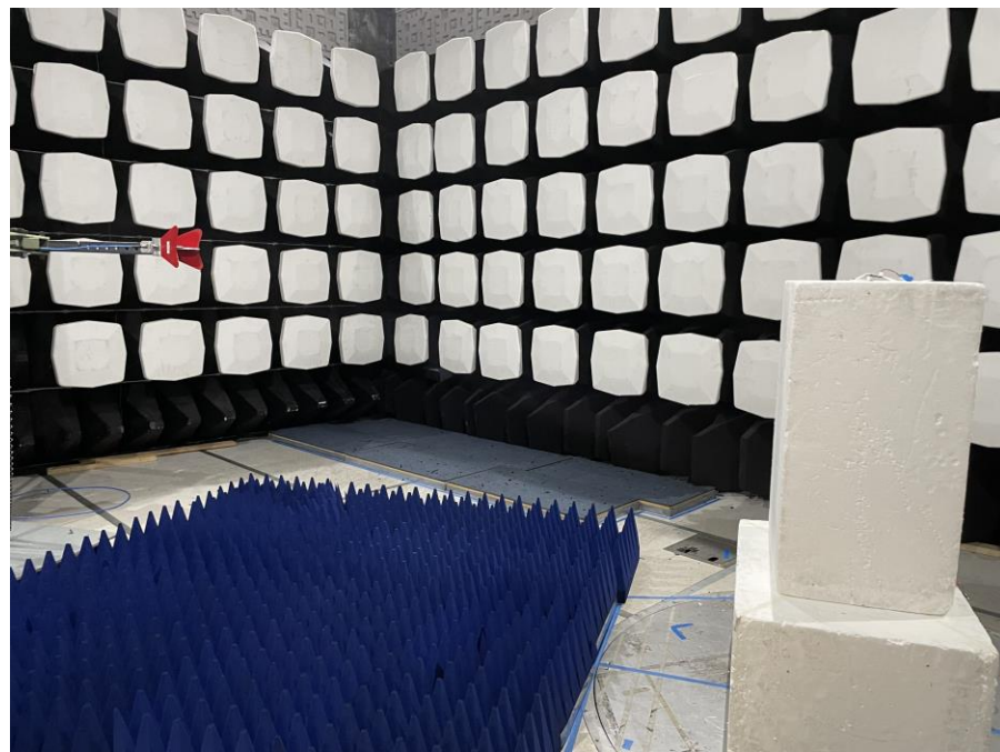
Figure 6: Equipment Under Test – Radiated Emissions >1GHz
