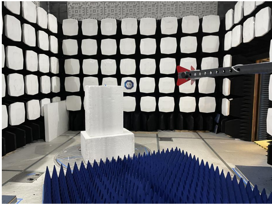
Figure 5: Equipment Under Test – Radiated Emissions >1GHz
