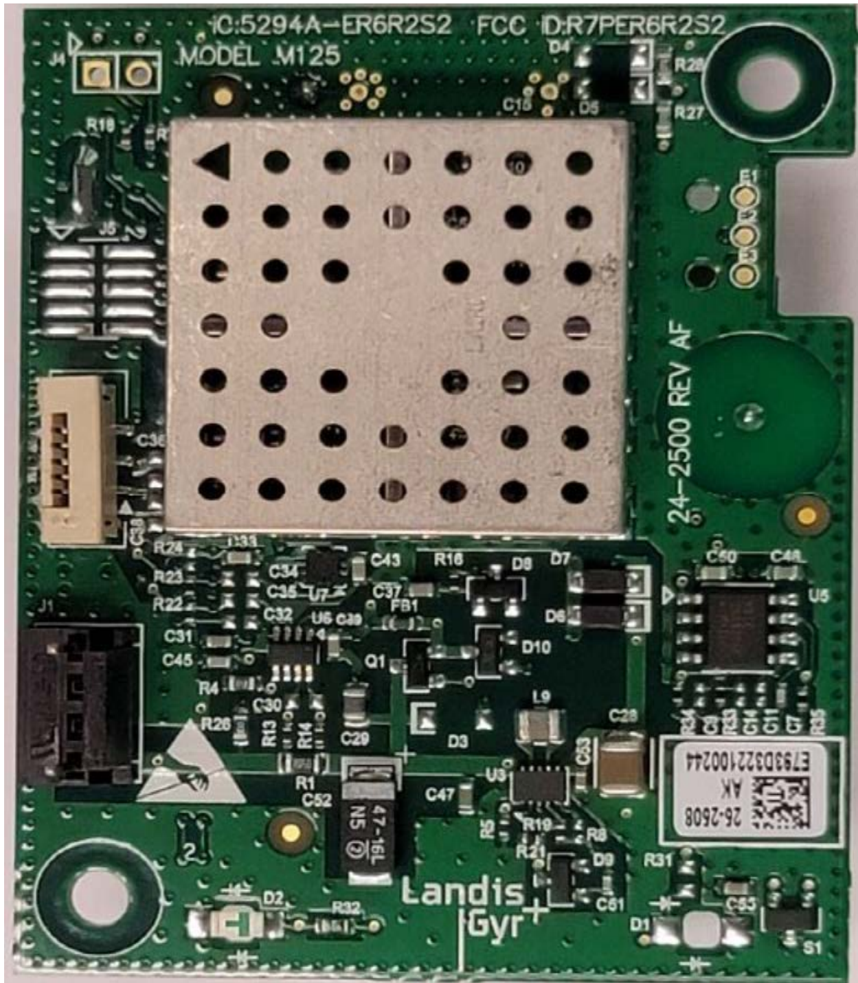
Figure 1: Top View
