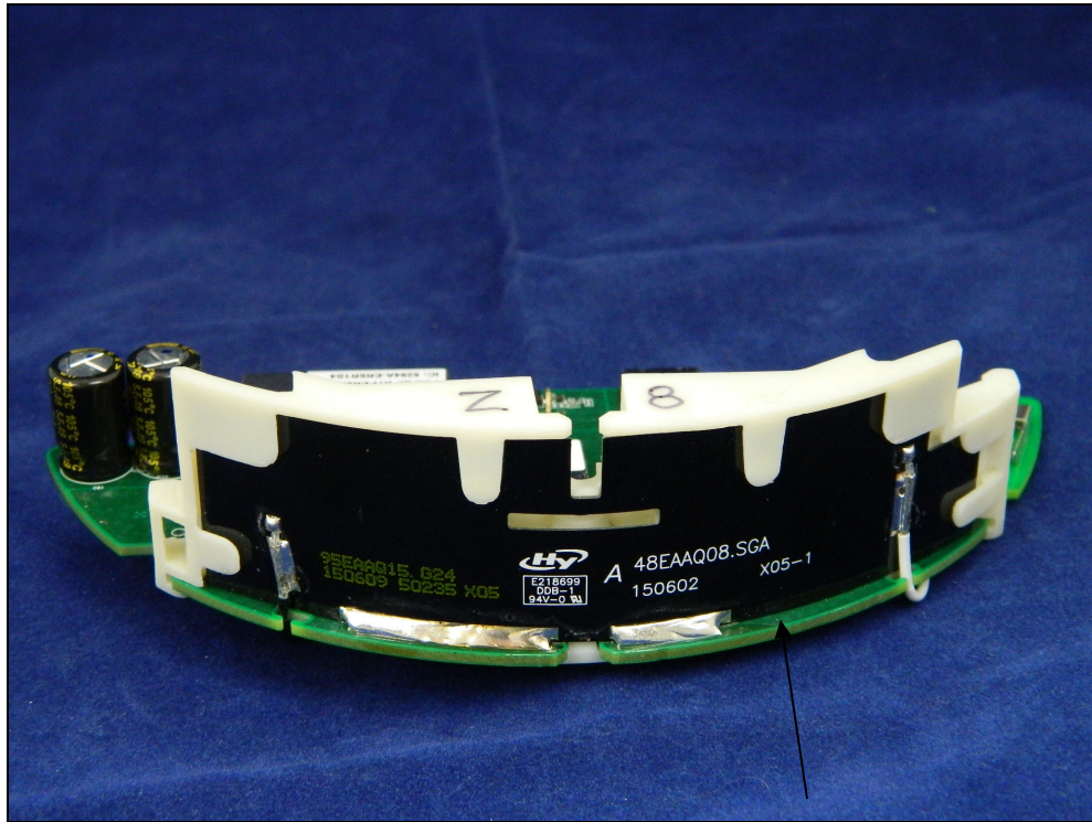
Figure 3: External Photo – Cellular Antenna
