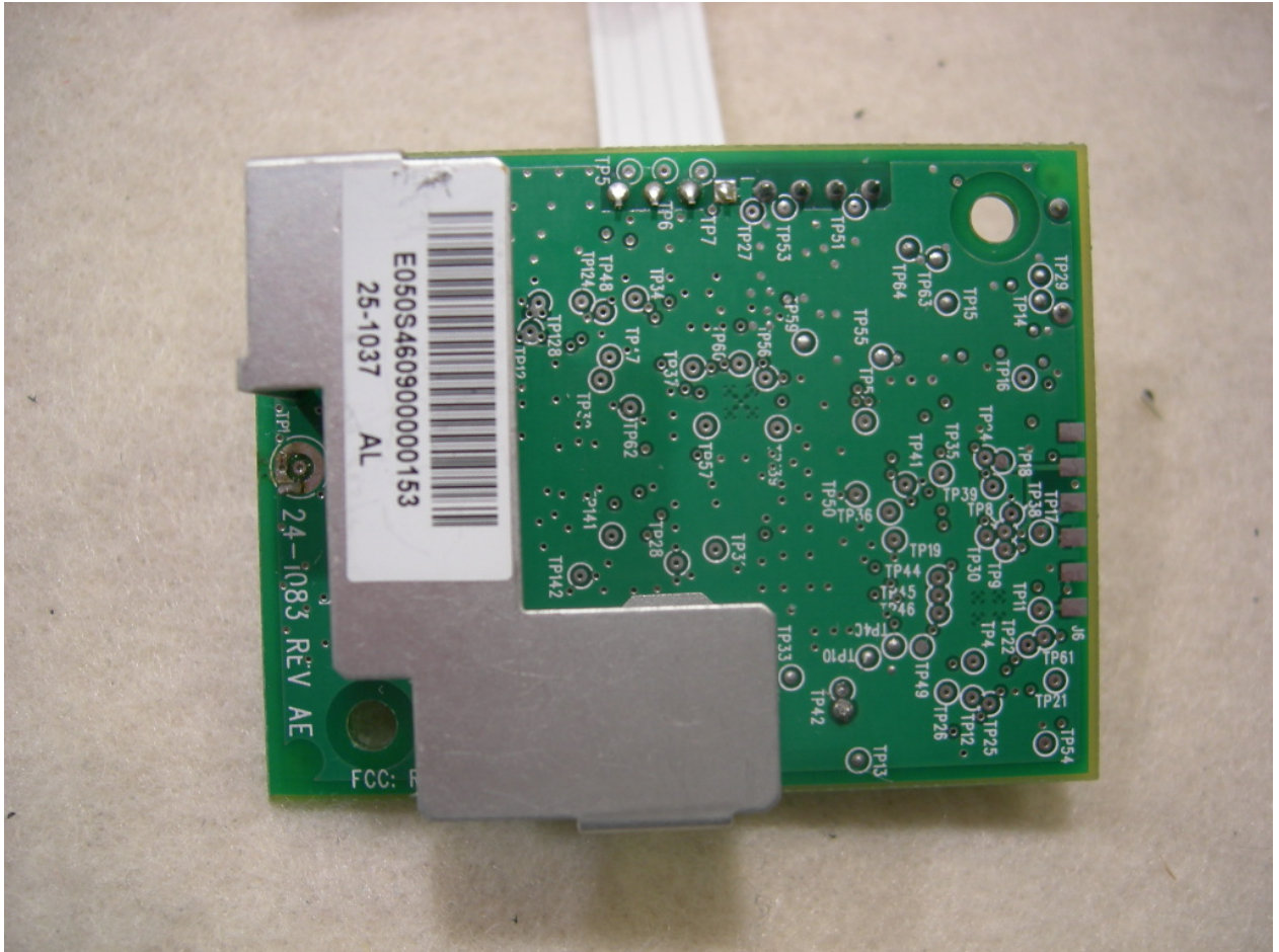
Figure 4: PCB - Back
