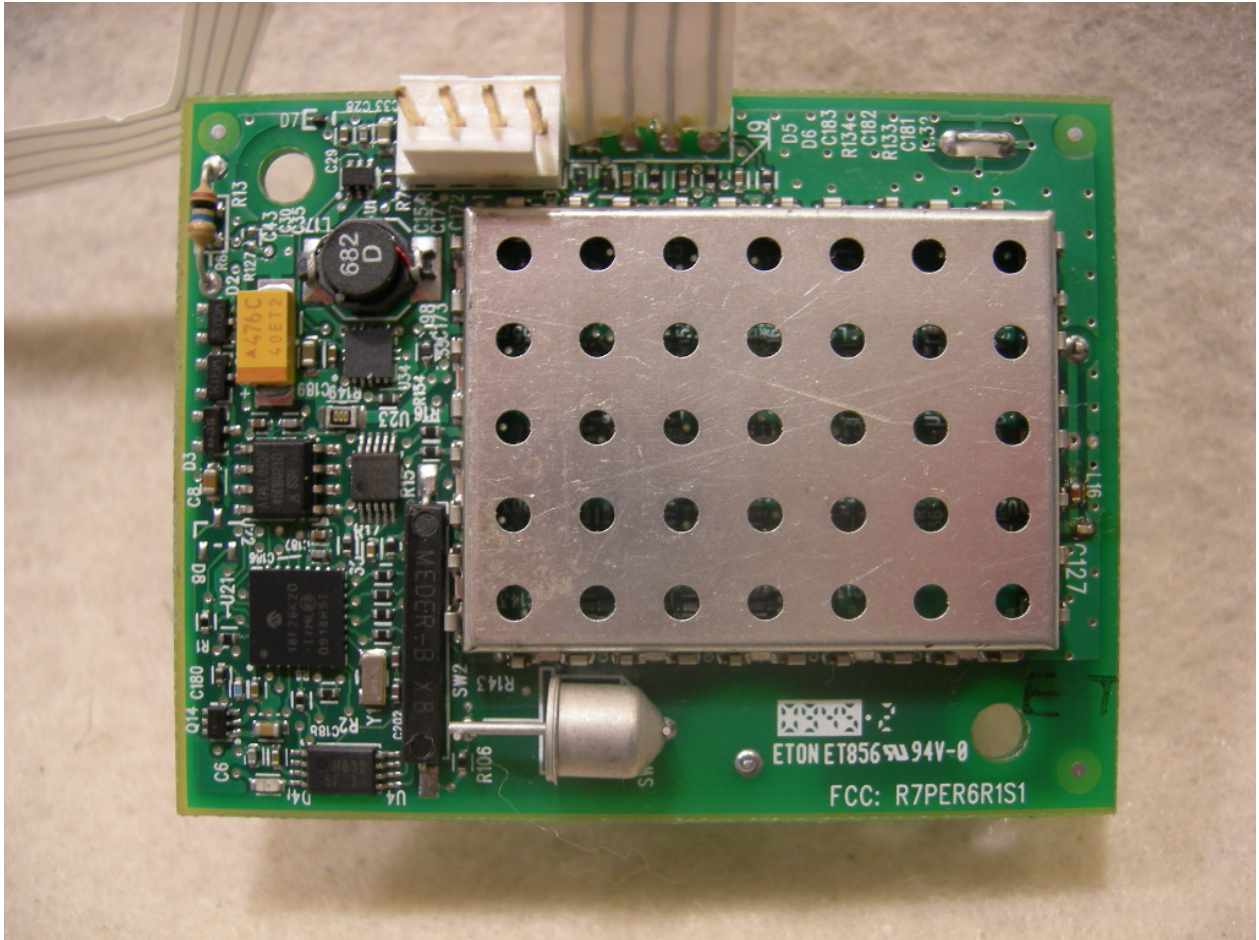
Figure 2: PCB with Shields – Front
