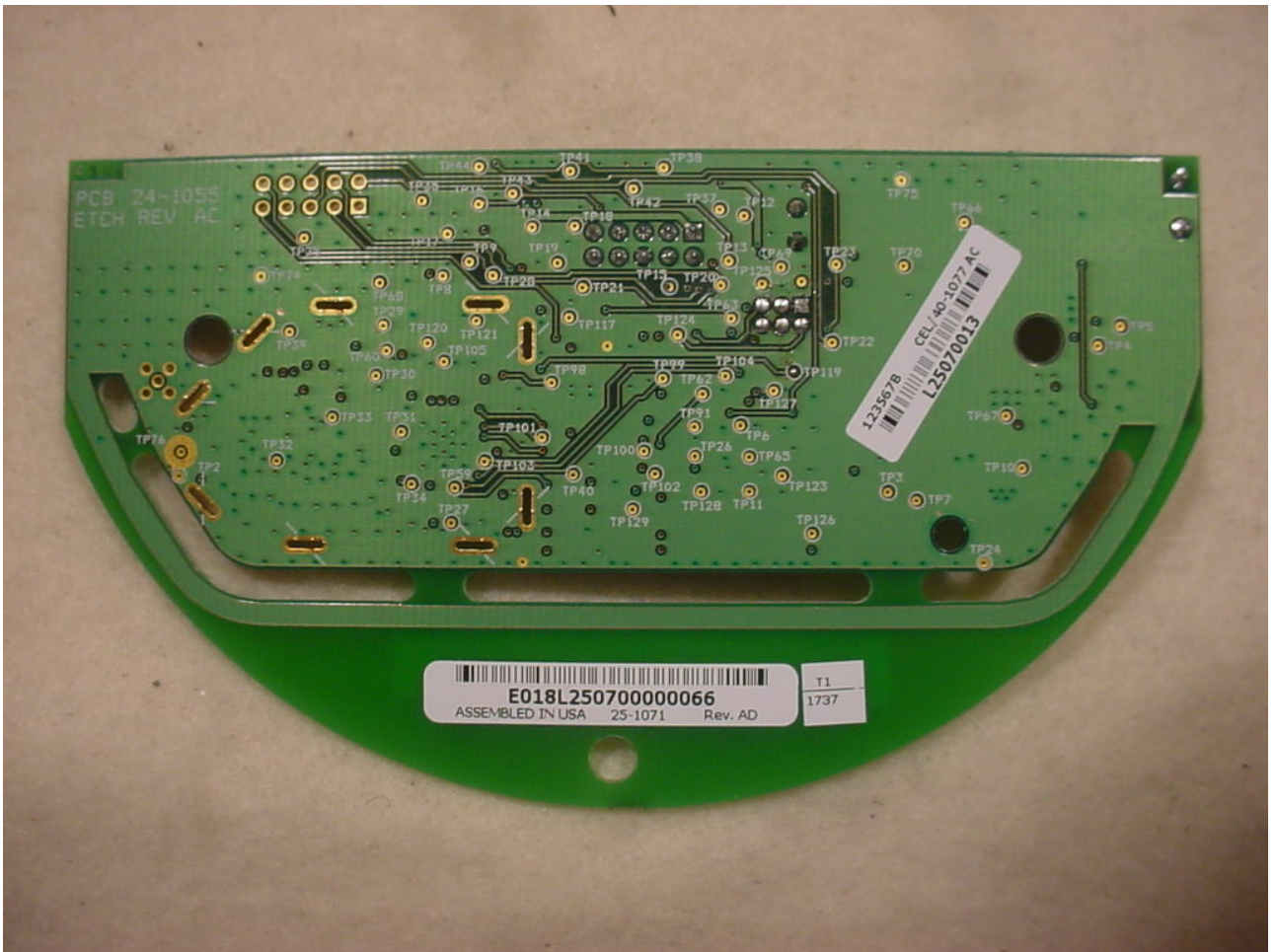
Figure 4: Utilinet 900 MHz PCB – Bottom View
