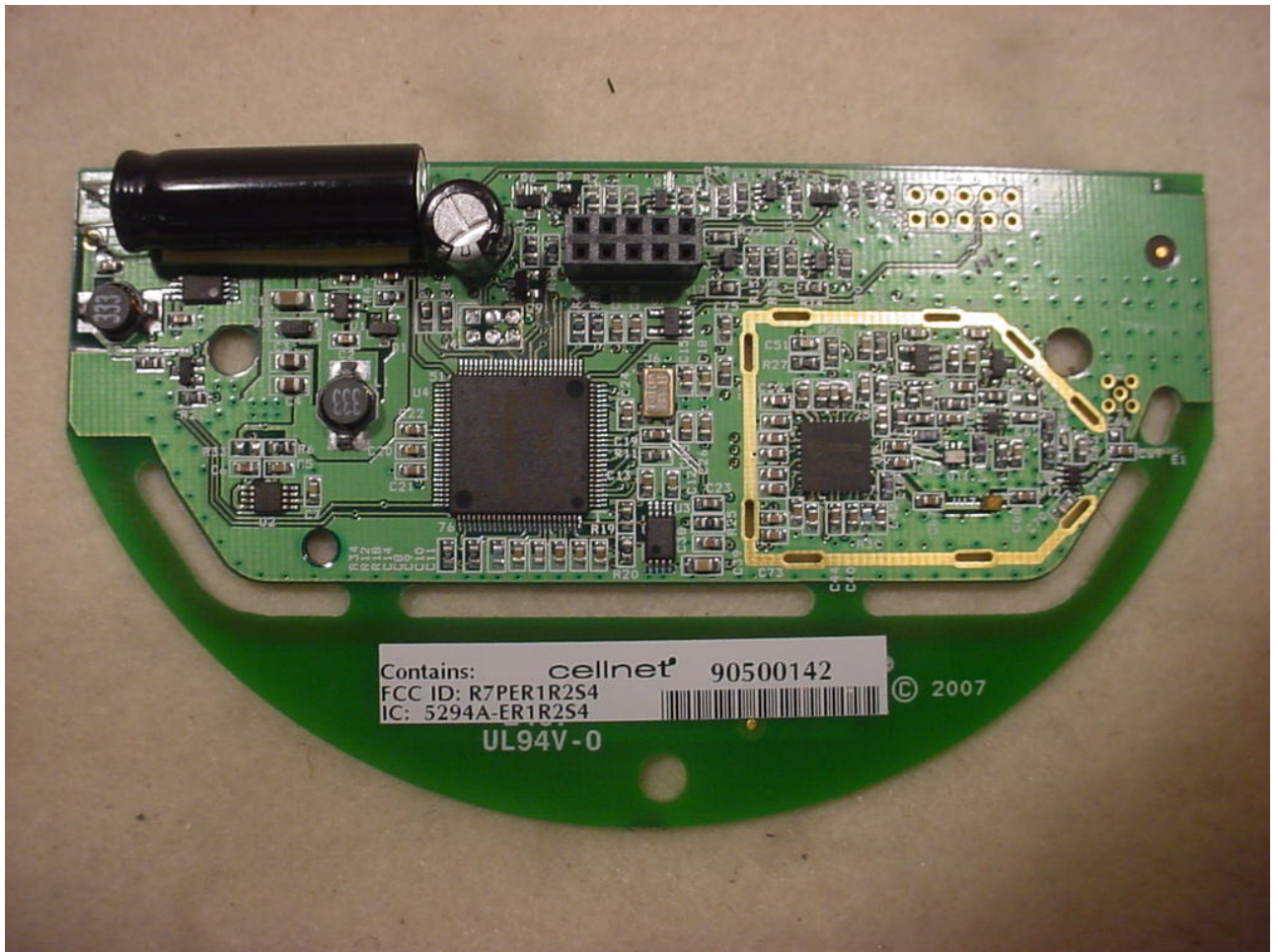
Figure 3: Utilinet 900 MHz PCB – Tops View
