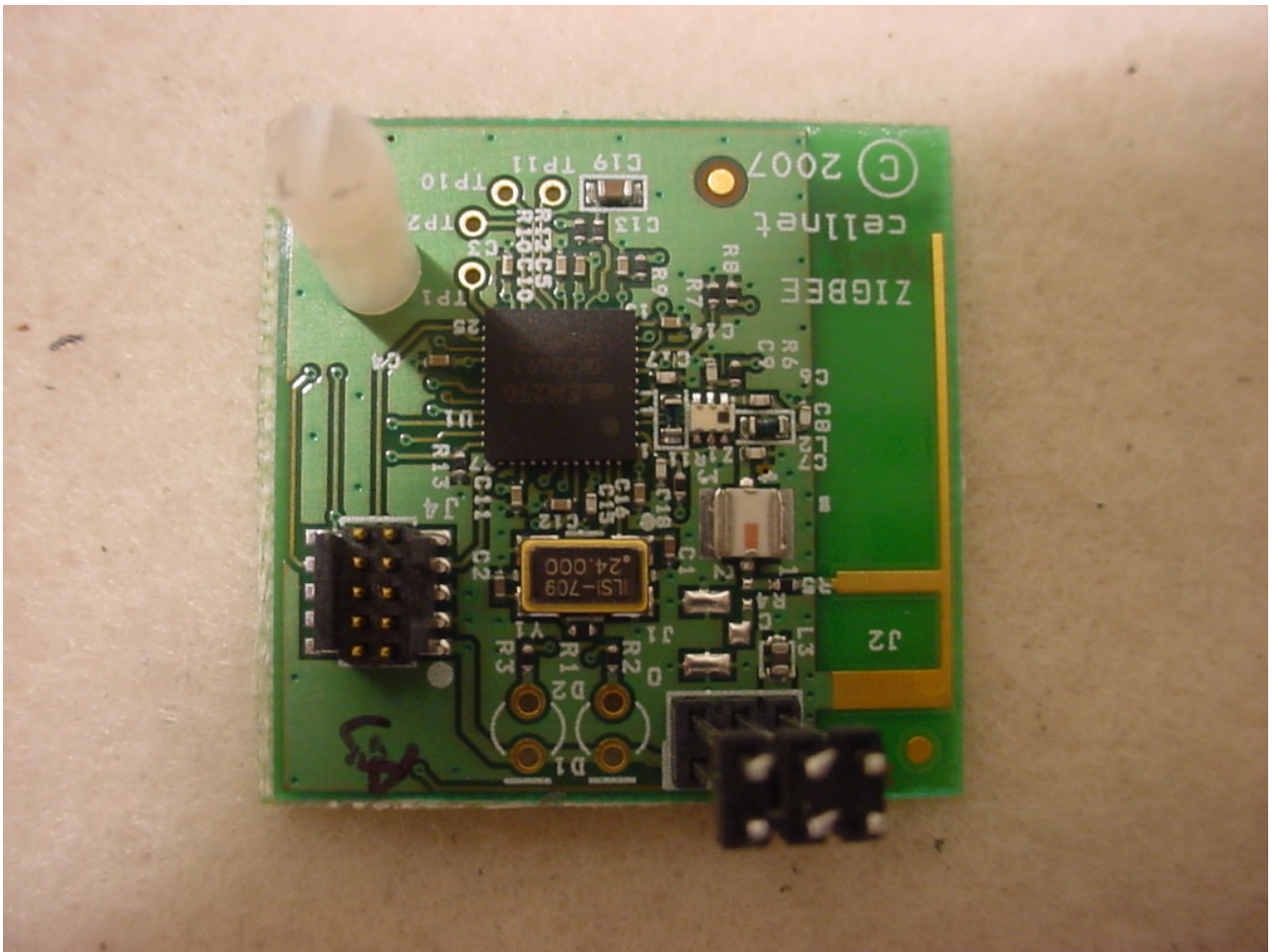
Figure 6: Zigbee 2400 MHz PCB – Bottom View
