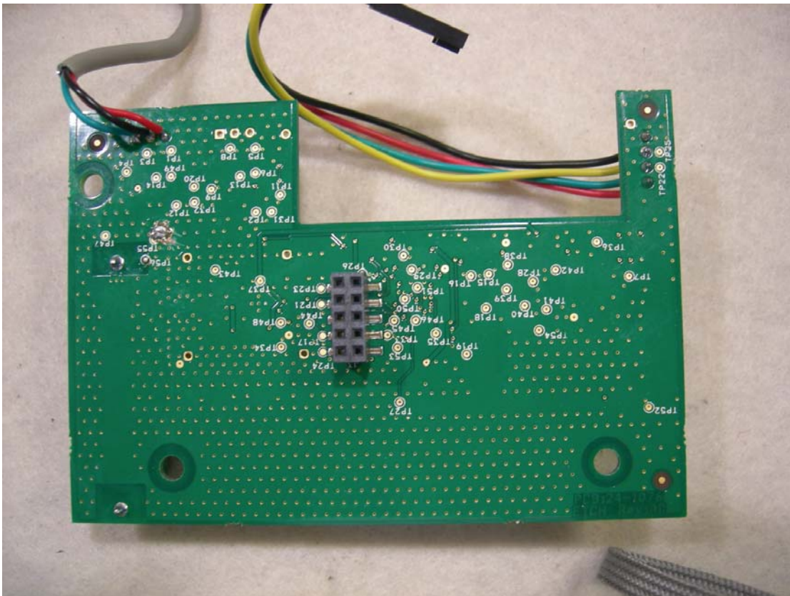
Figure 3: PCB - Back
