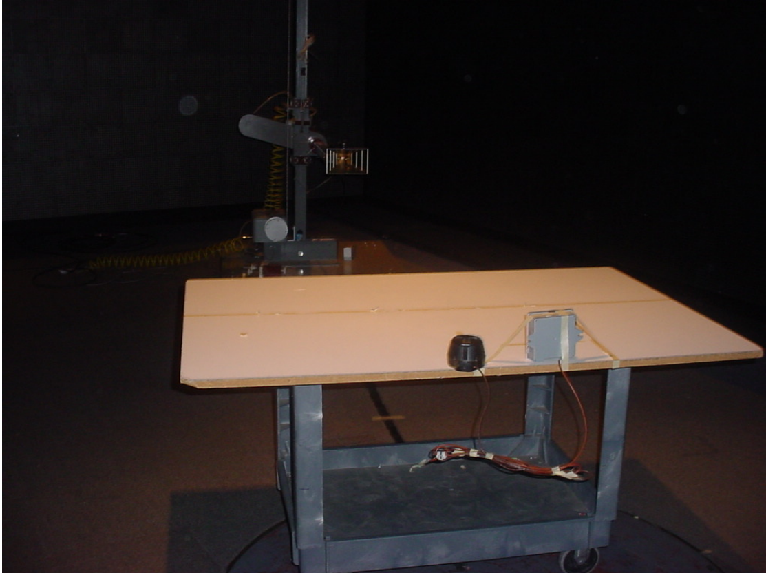
Figure2: Intentional Radiated Emissions
