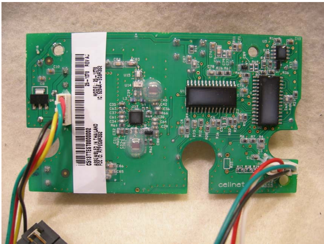
Figure 1: PCB – Front
