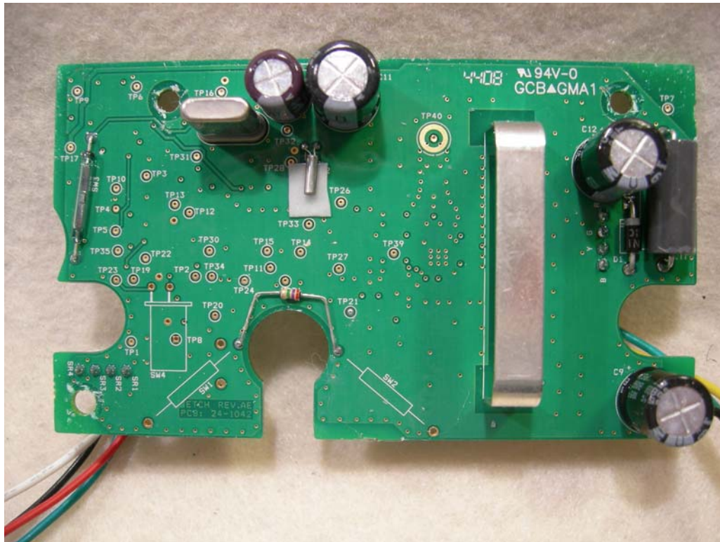
Figure 2: PCB - Back
