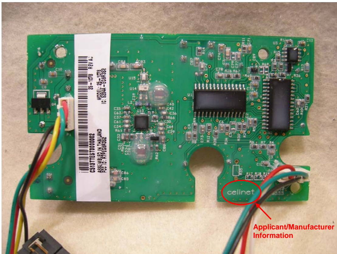
Figure 1: PCB – Label Location
