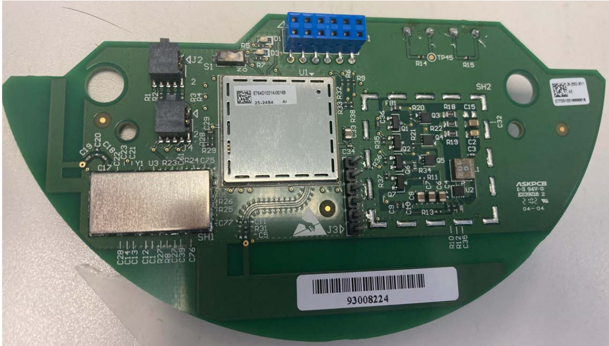
Figure 1: Top View
