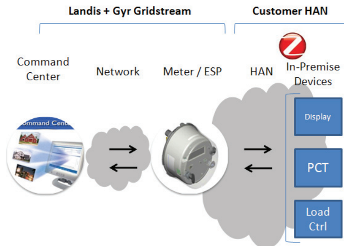
Figure 1 - 4. ZigBee Communication
