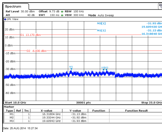
Figure 7.5.1.2-9: 10 GHz – 25 GHz – 2475 MHz
