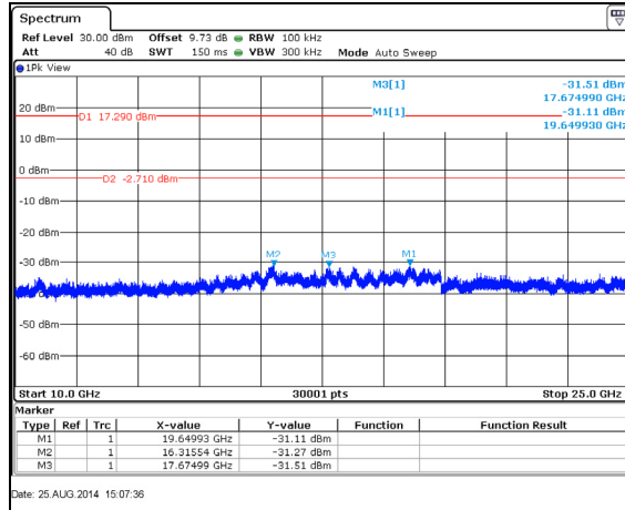
Figure 7.5.1.2-6: 10 GHz – 25 GHz – 2445 MHz
