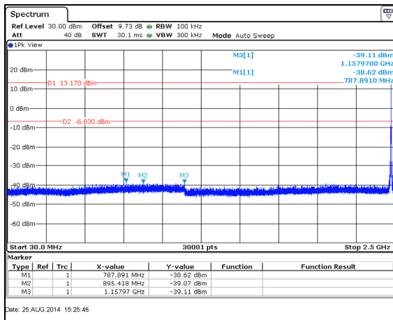
Figure 7.5.1.2-7: 30 MHz – 2.5 GHz – 2475 MHz
