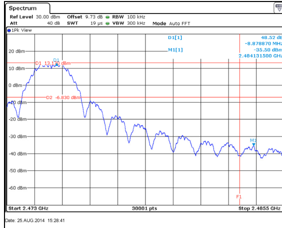
Figure 7.5.1.2-11: Upper Band-edge - 2475 MHz
