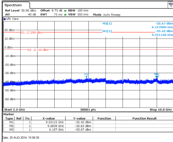
Figure 7.5.1.2-5: 2.5 GHz – 10 GHz – 2445 MHz
