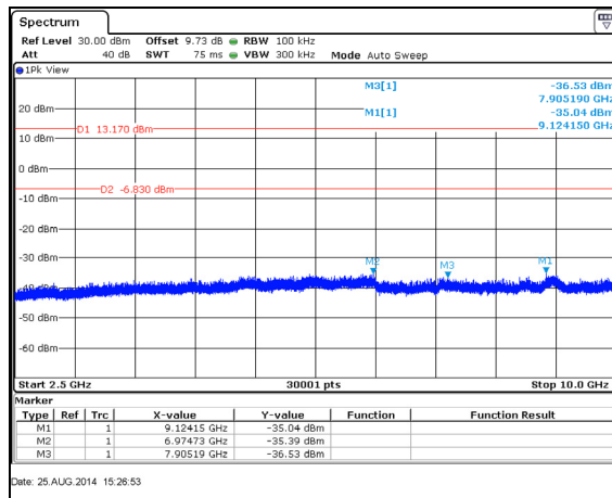
Figure 7.5.1.2-8: 2.5 GHz – 10 GHz – 2475 MHz
