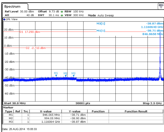
Figure 7.5.1.2-4: 30 MHz – 2.5 GHz – 2445 MHz
