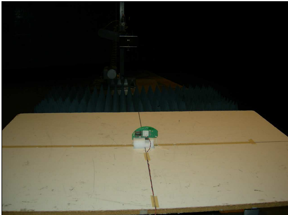
Figure 2: Radiated Emissions
