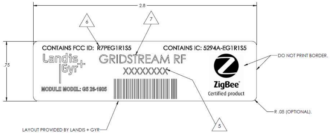
Figure 4: Sample Host Label
