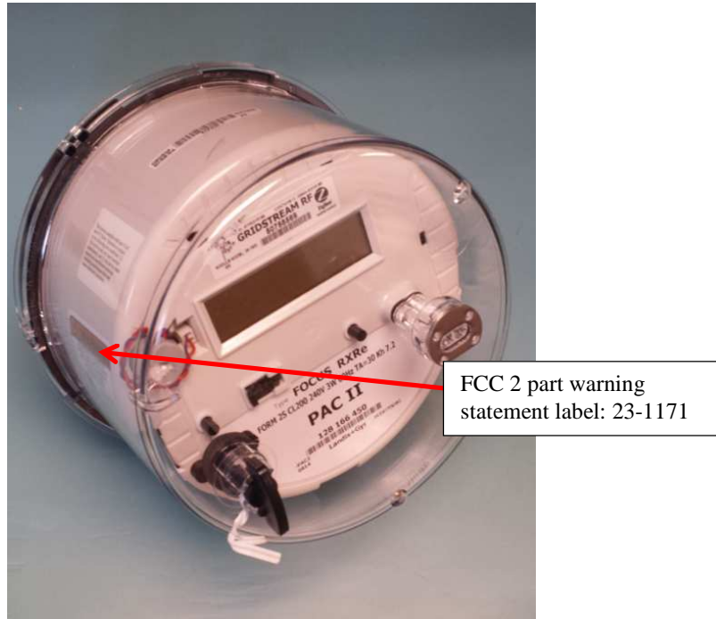
Figure 6: Sample Host Label Placement
