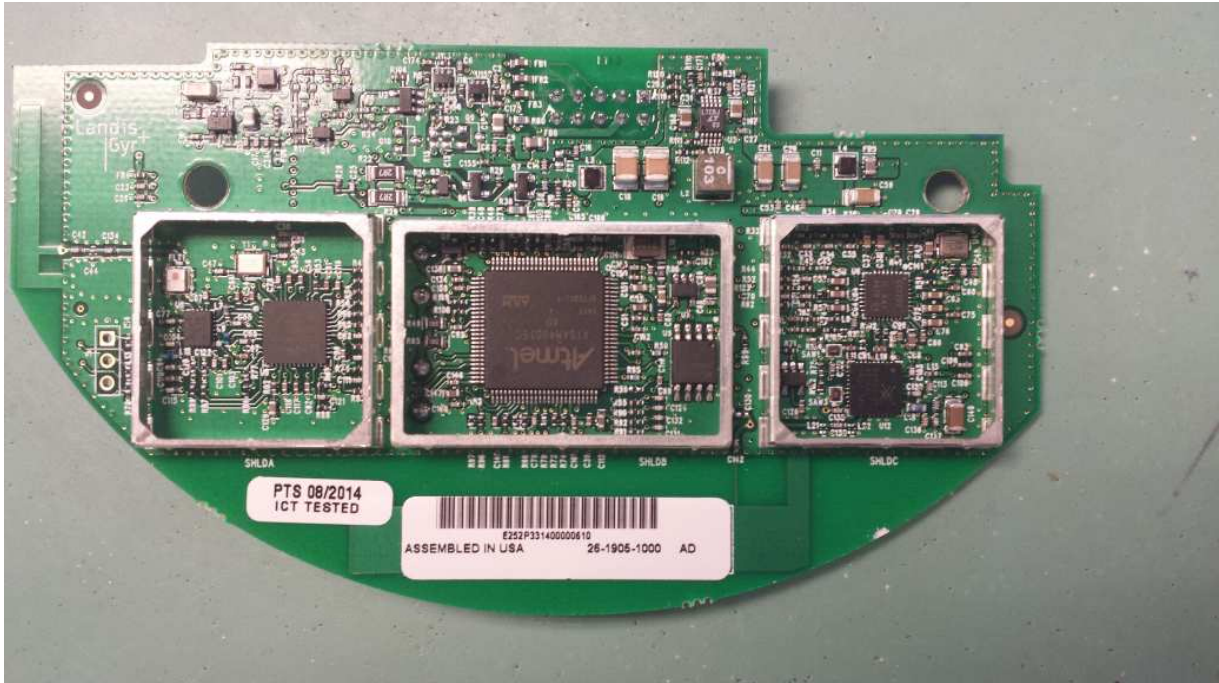
Figure 1: Internal Photo – Shields Removed
