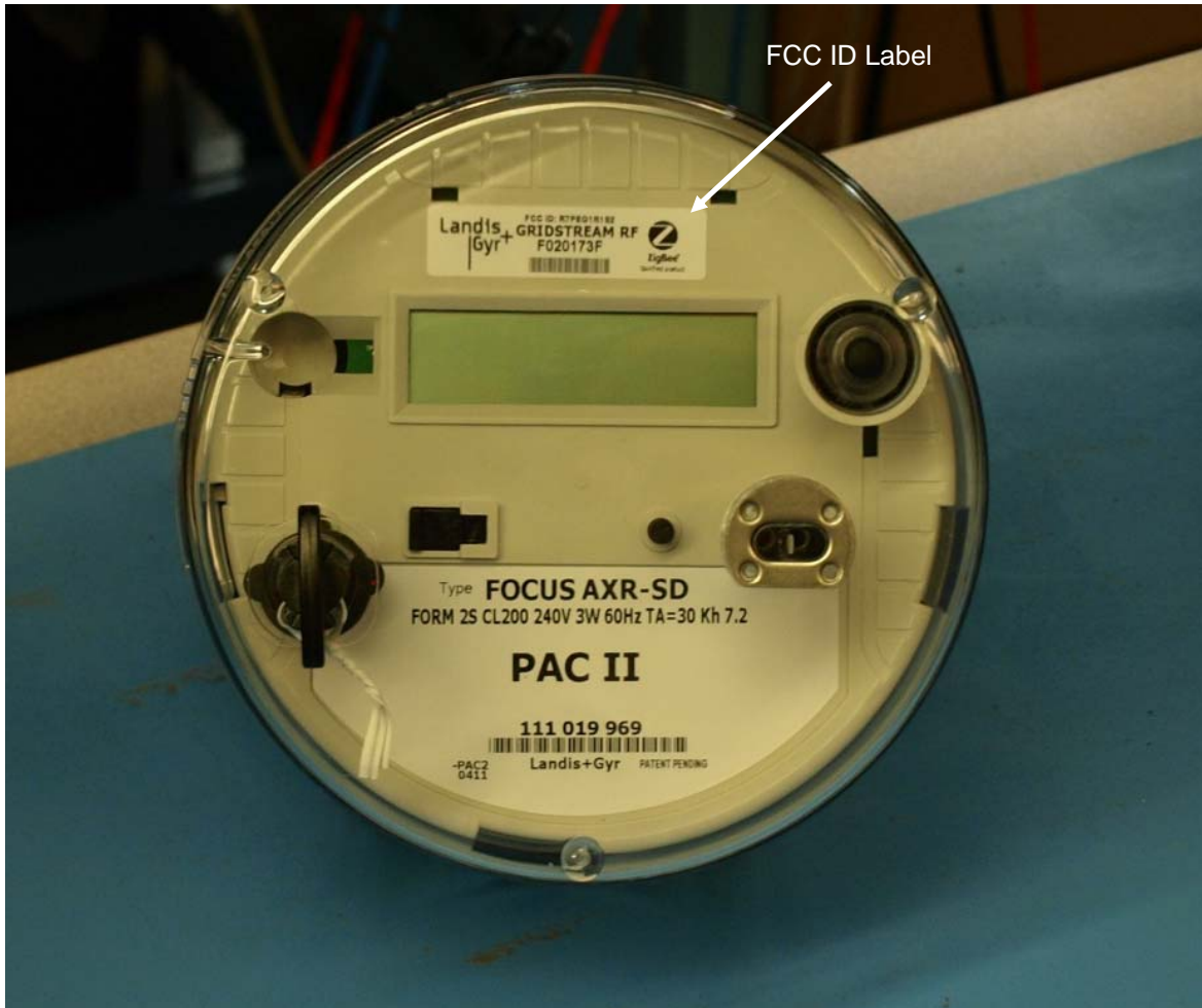
Figure 3: Identifier Label Location
