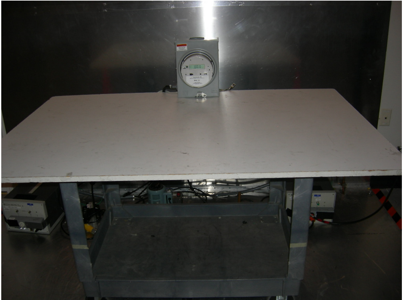
Figure 5: Conducted Emissions
